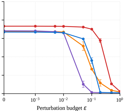
(b) CIFAR-100
