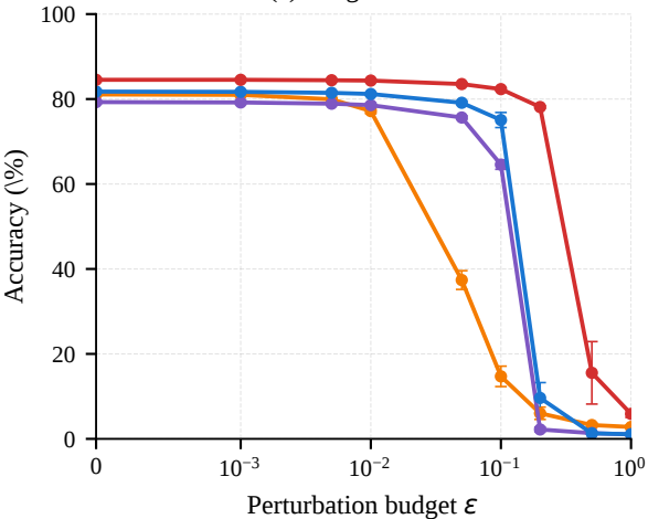
(a) ImageNet-100
