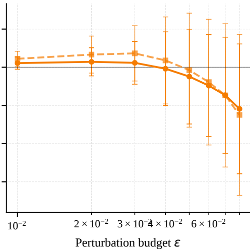
(b) CIFAR-100
