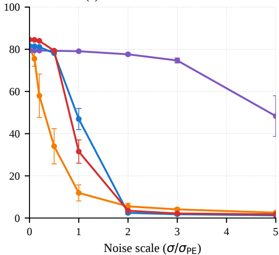
(a) Random Gaussian noise
