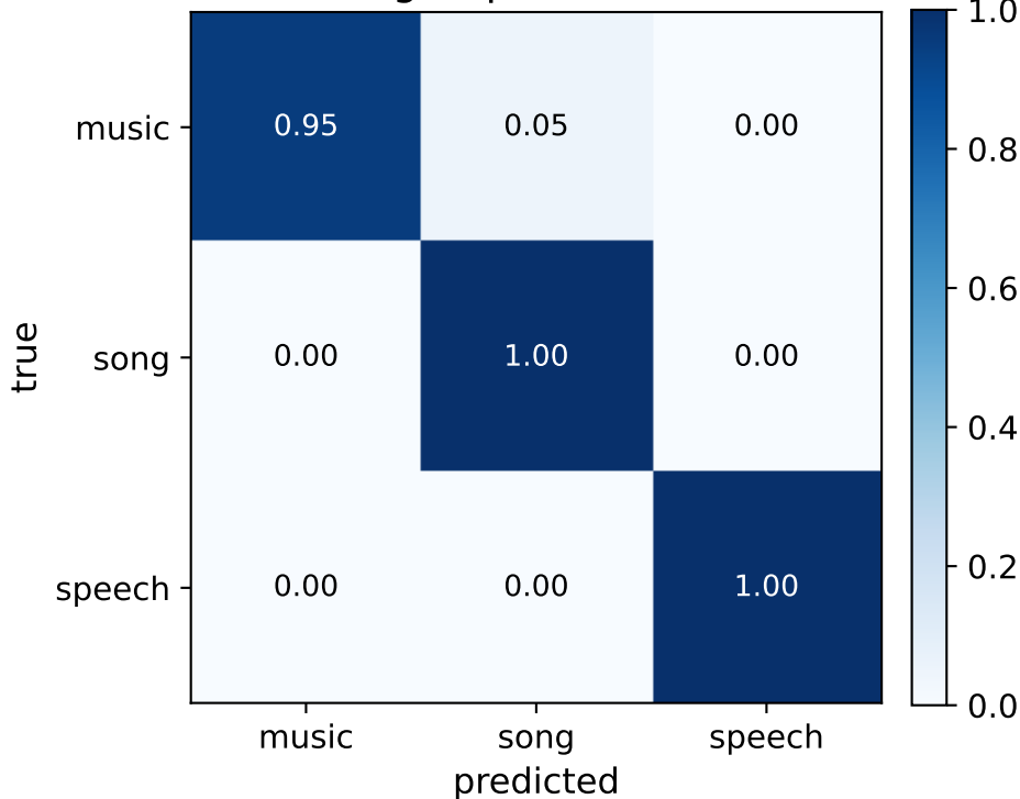
3-class decoder (grouped CV, window (0.2, 0.6))
