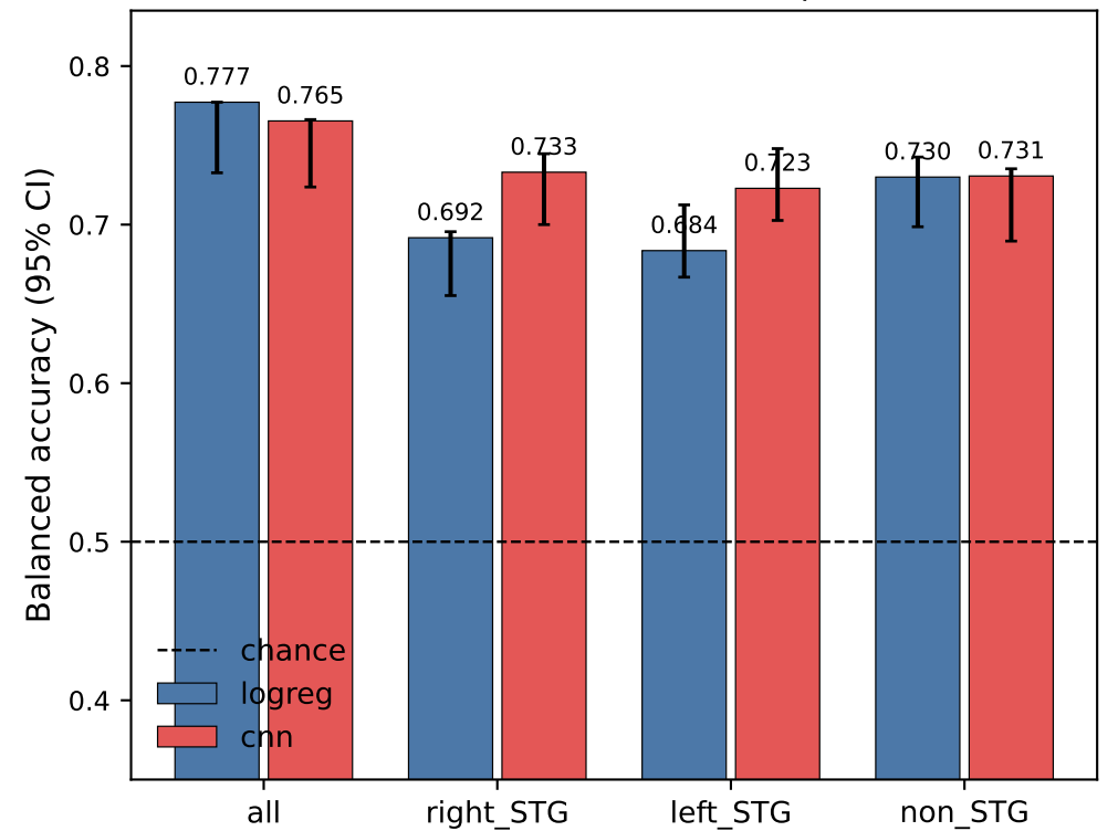
Bellier vocal vs instrumental decoder (blocked 5-fold CV)
