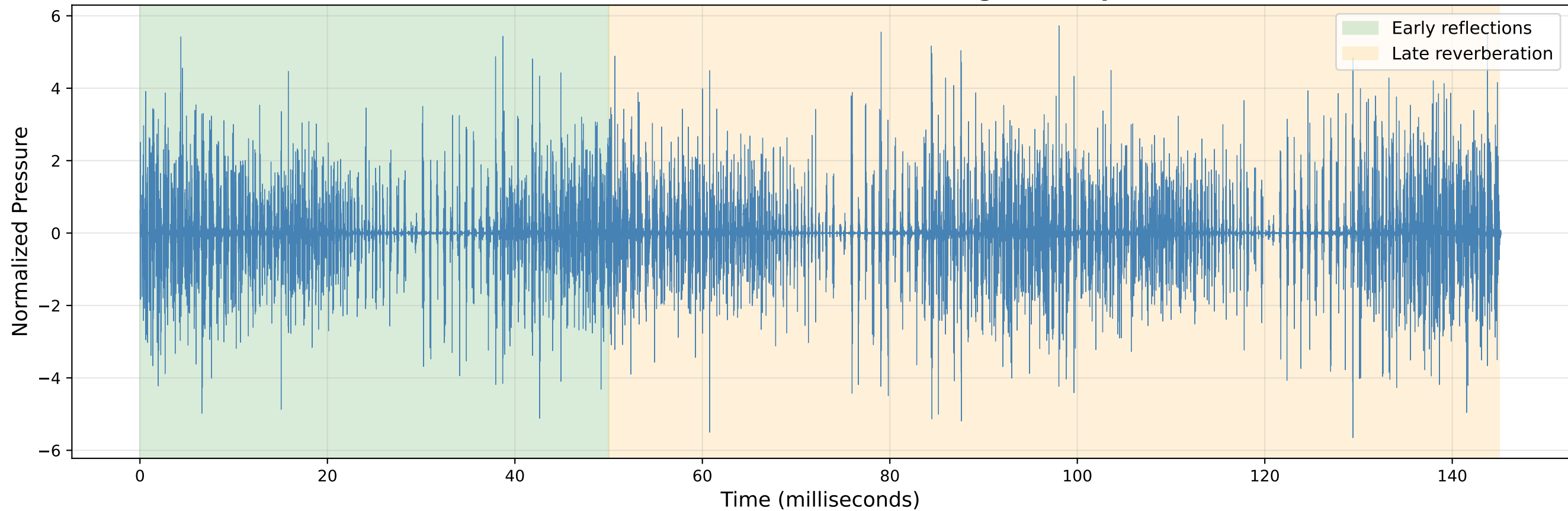
Raw Acoustic Pressure Time-Series (Single Microphone)
