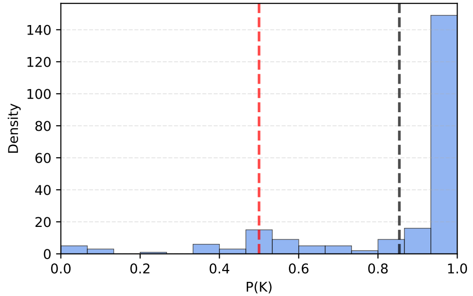
J(K vs R) - Combined \mu : 0.854 | Obj: 0.500 | n=228
