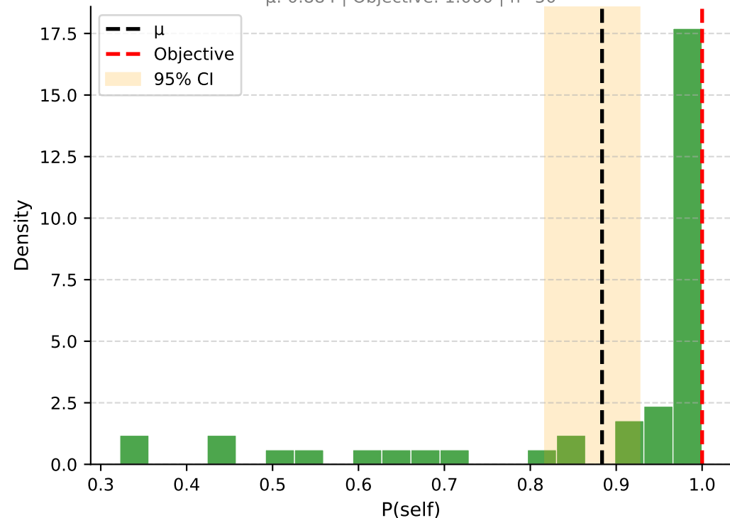
Legitimate Self-Preference (LSP)
