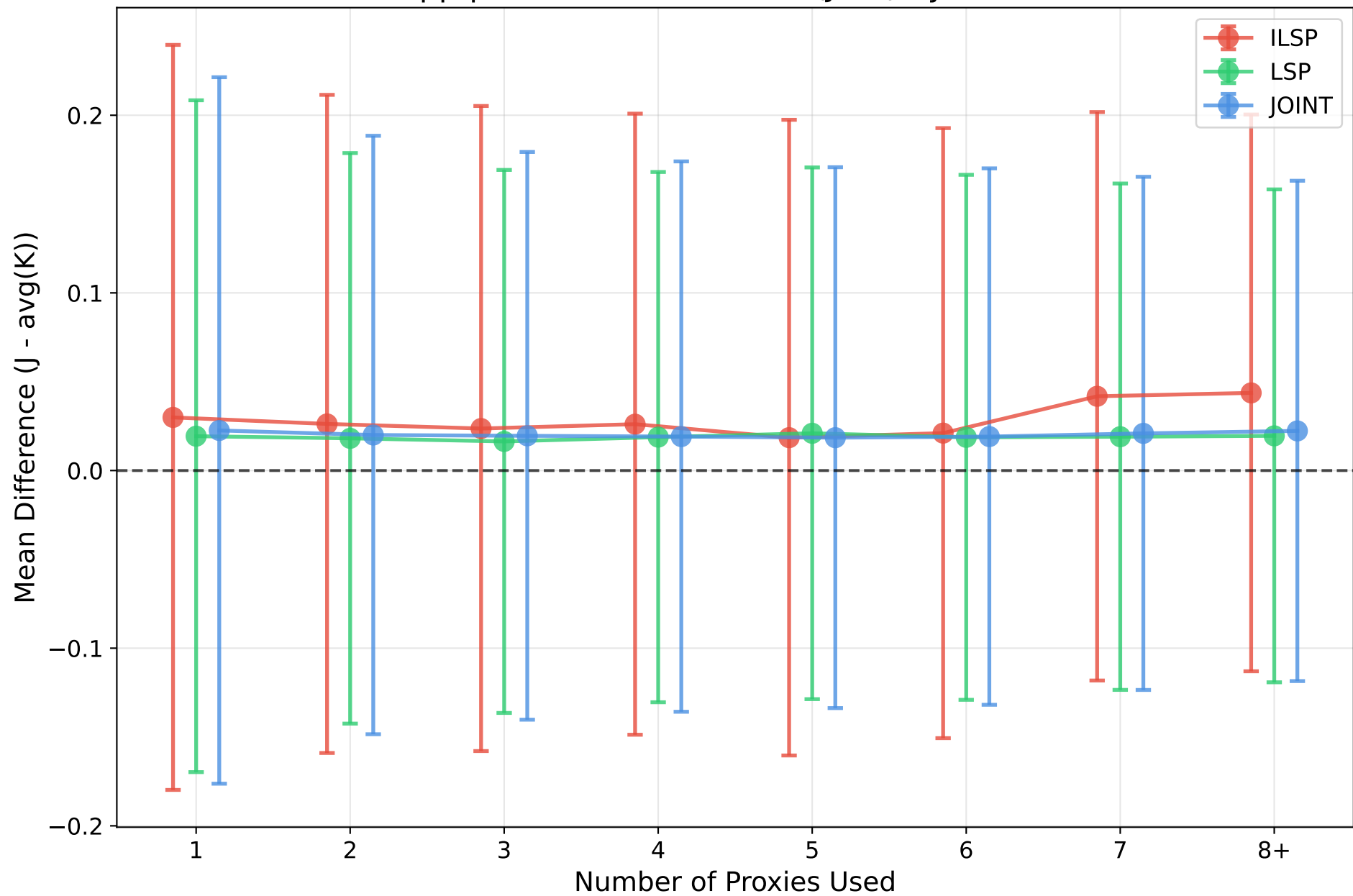
mbpp-plus: Mean Difference (J - K) by # Proxies
