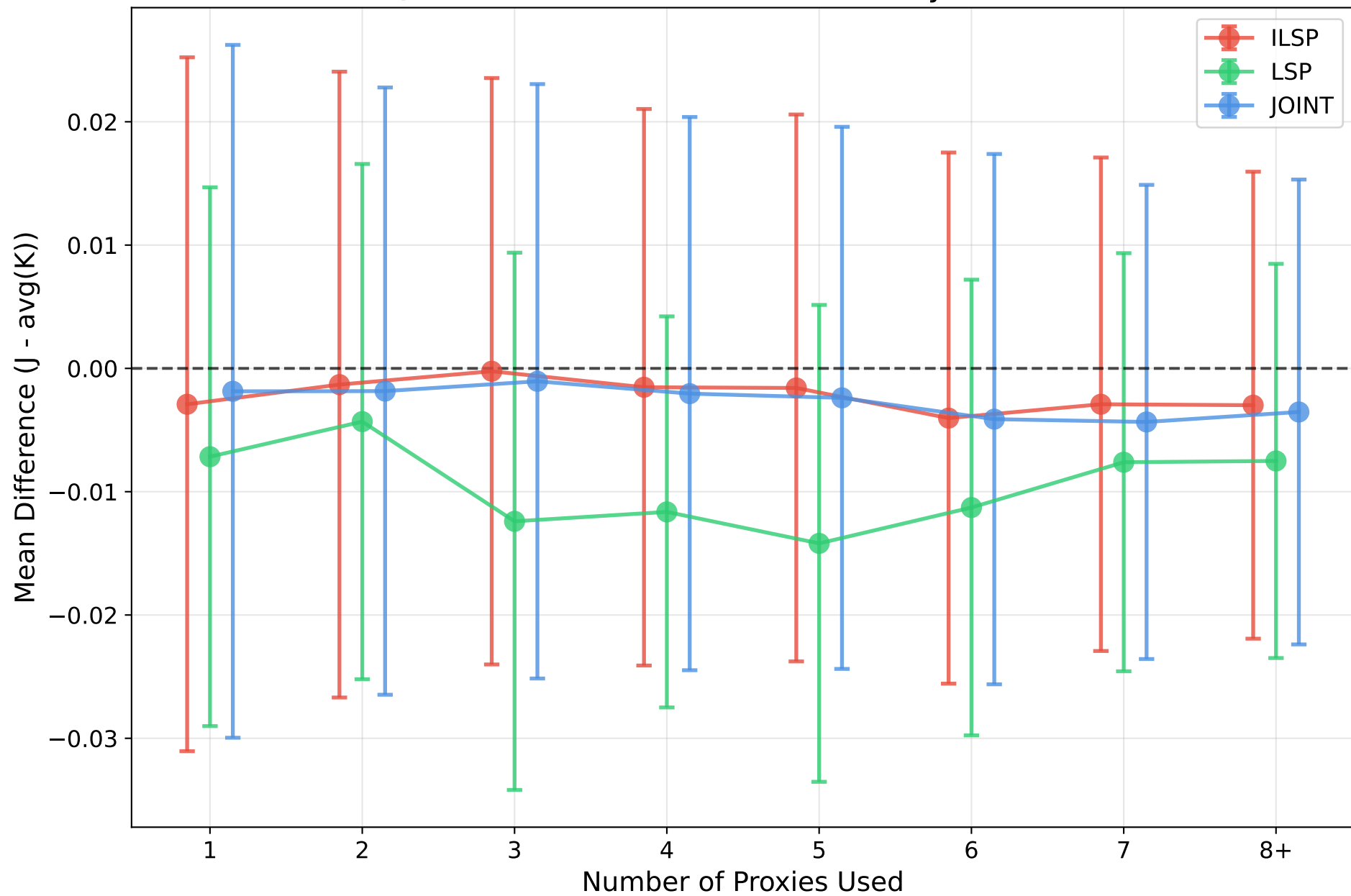
Qwen2.5-0.5B-Instruct: Mean Diff by # Proxies
