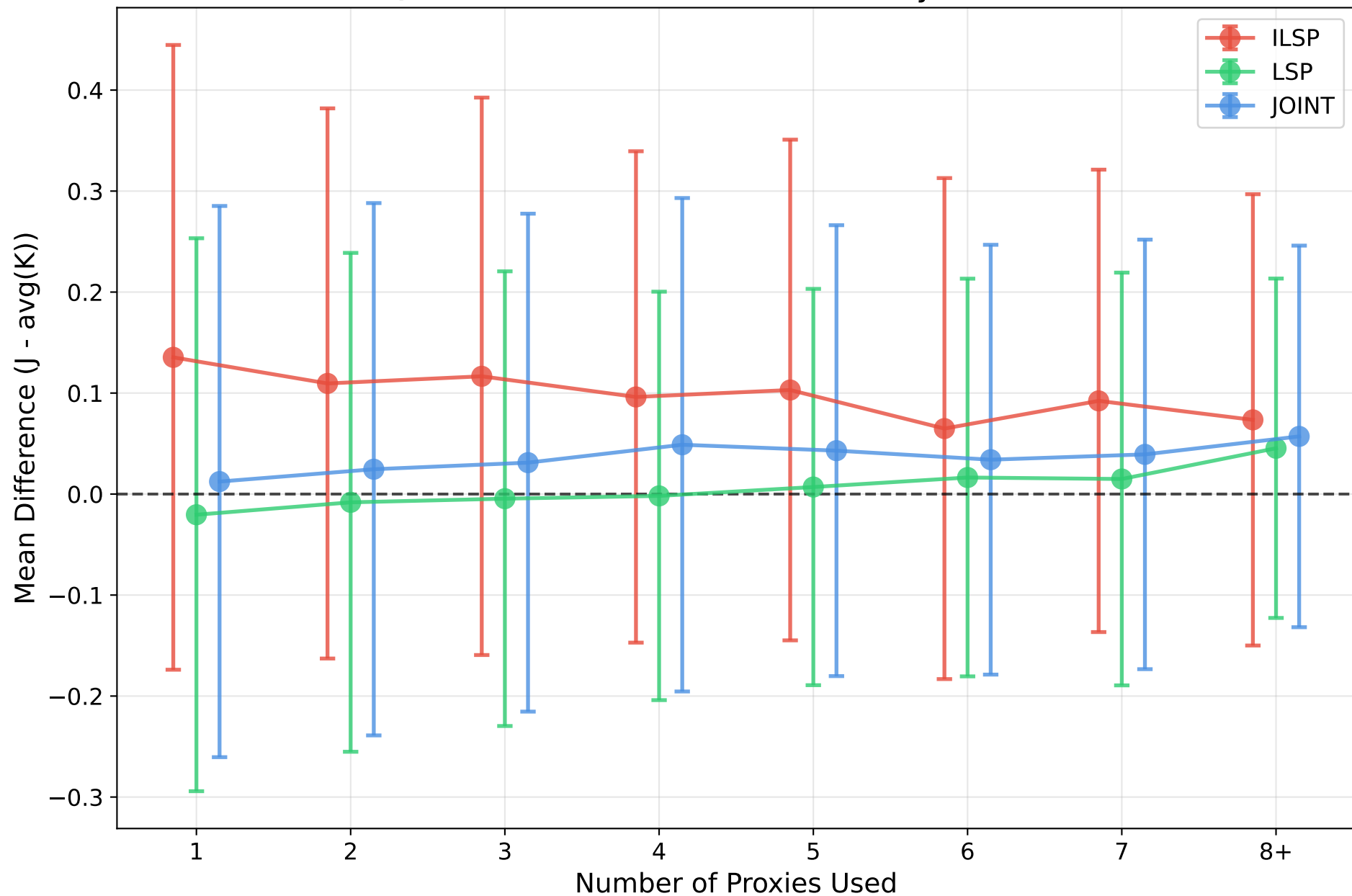
Qwen2.5-14B-Instruct: Mean Diff by # Proxies
