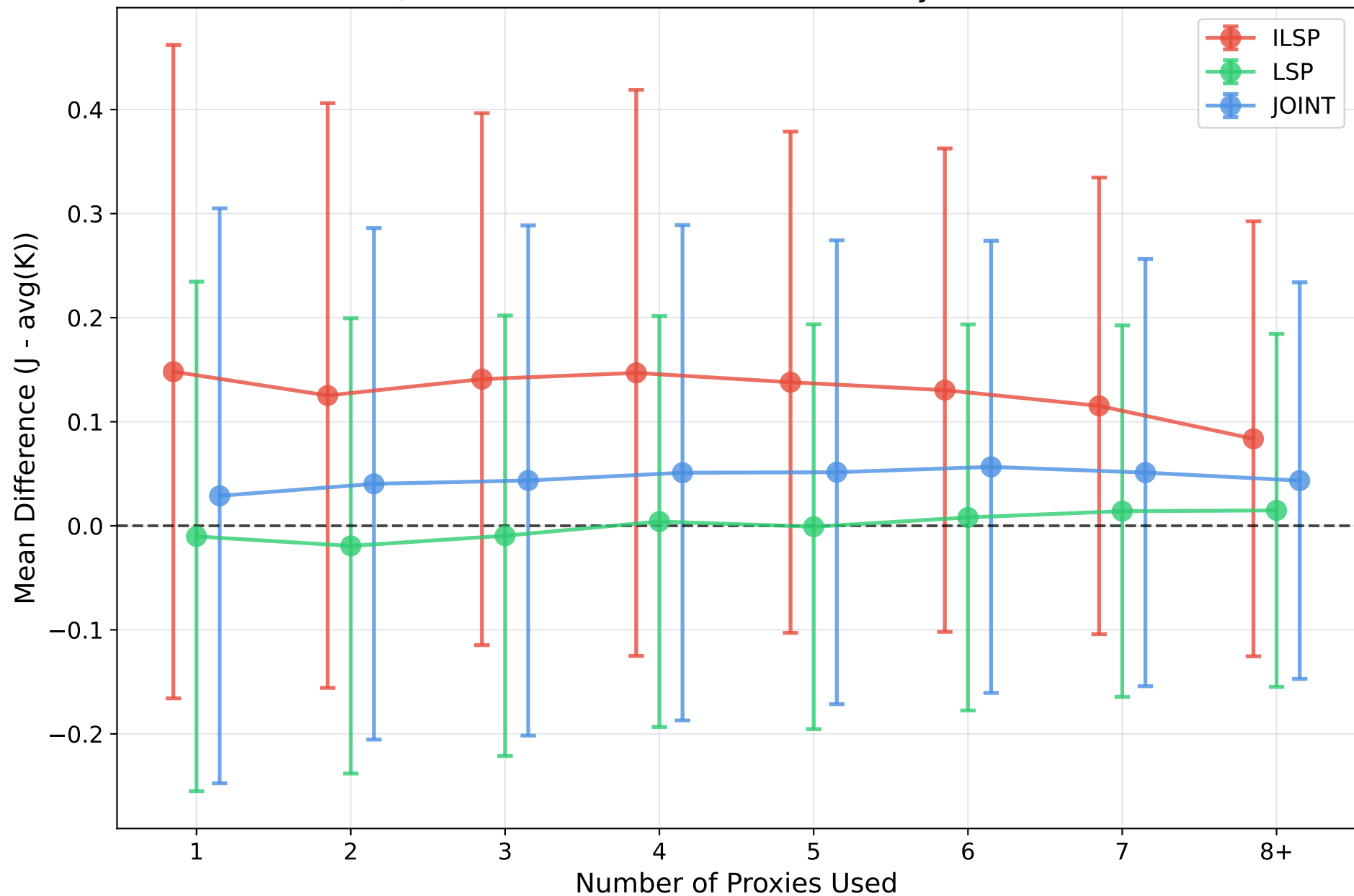
Qwen2.5-32B-Instruct: Mean Diff by # Proxies
