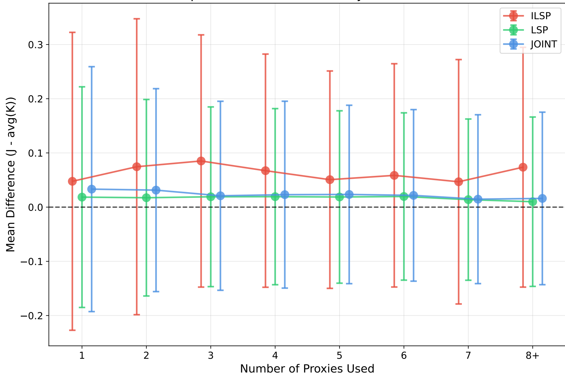
qwen-2.5-14b: Mean Diff by # Proxies
