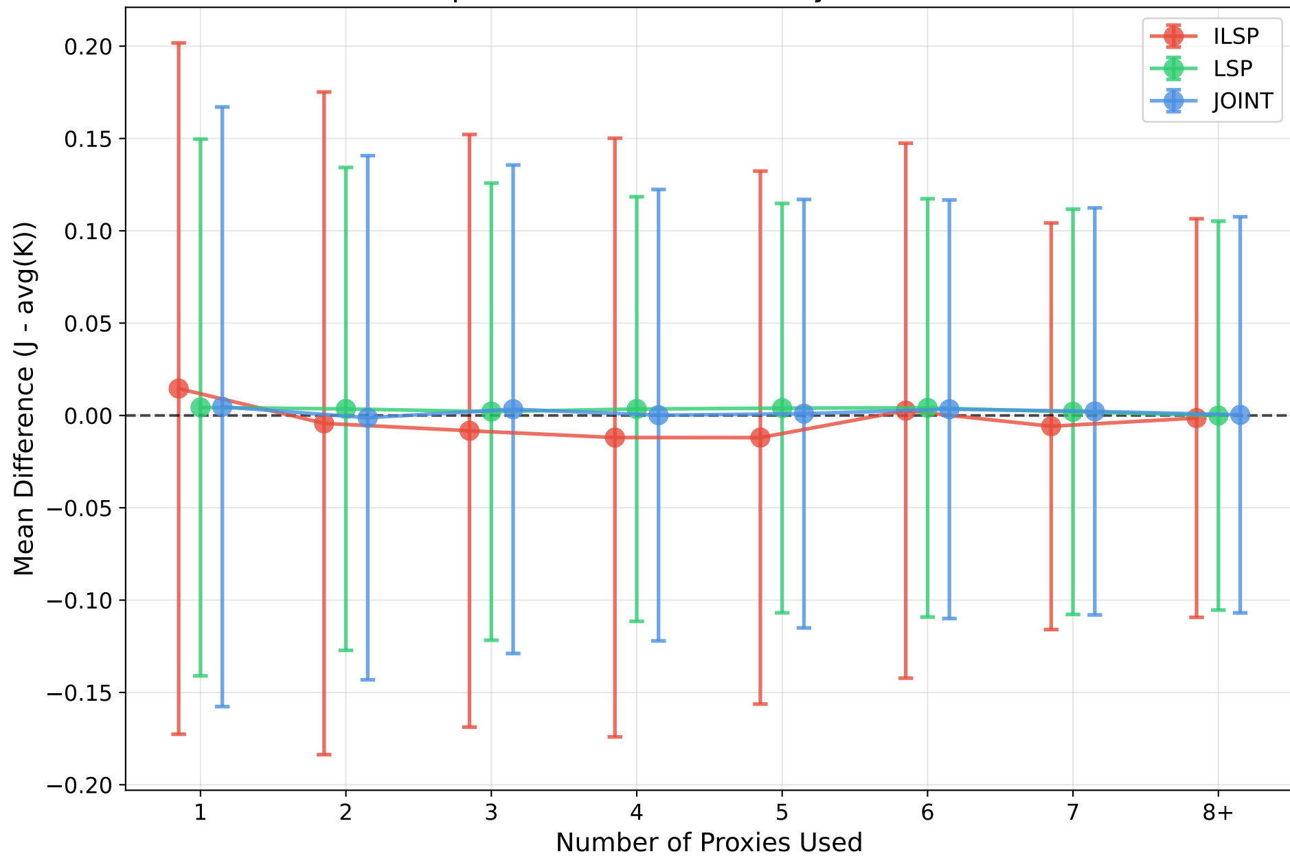
qwen-2.5-3b: Mean Diff by # Proxies
