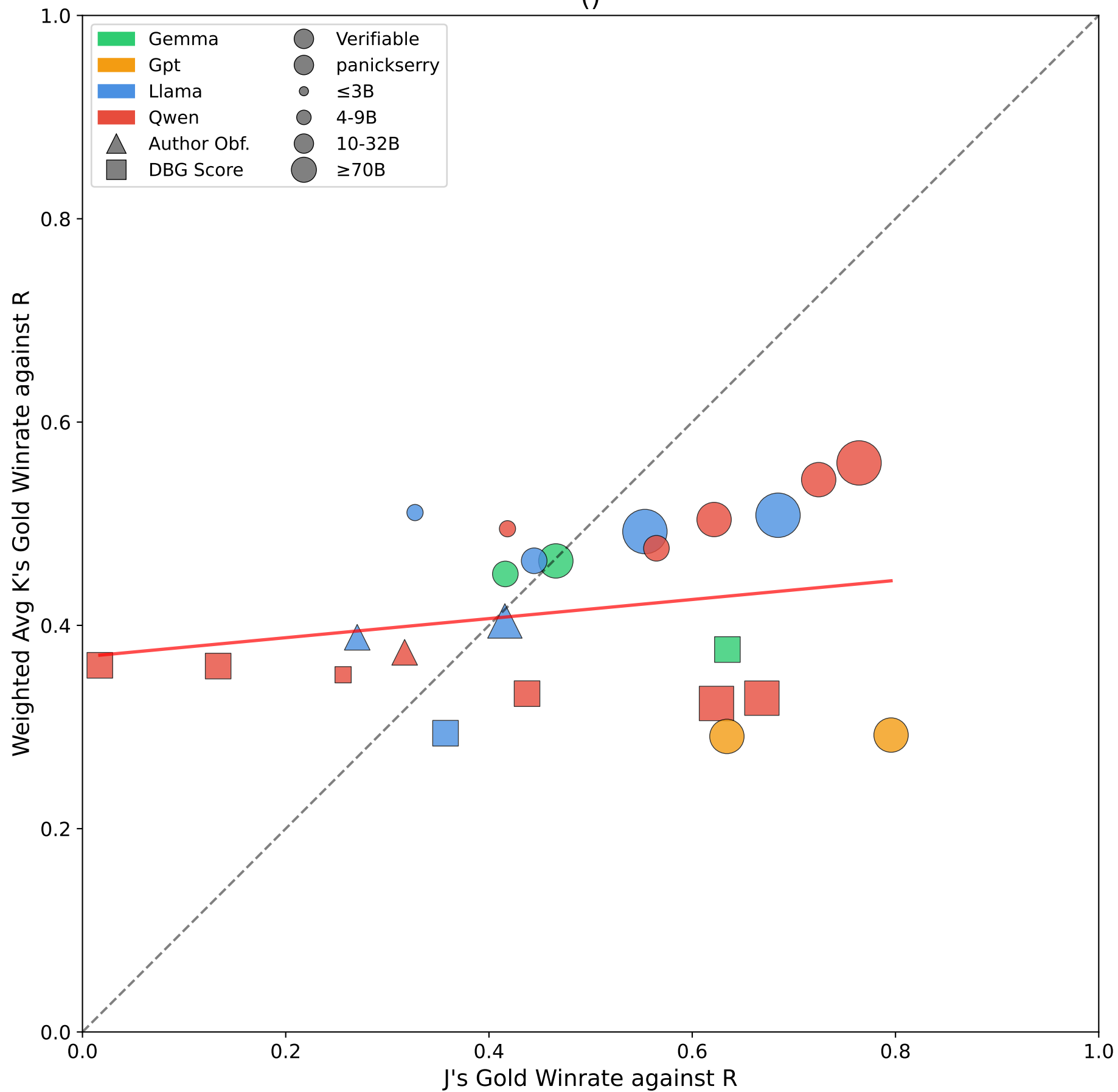
Gold Winrate Balance (by judge) ( )
