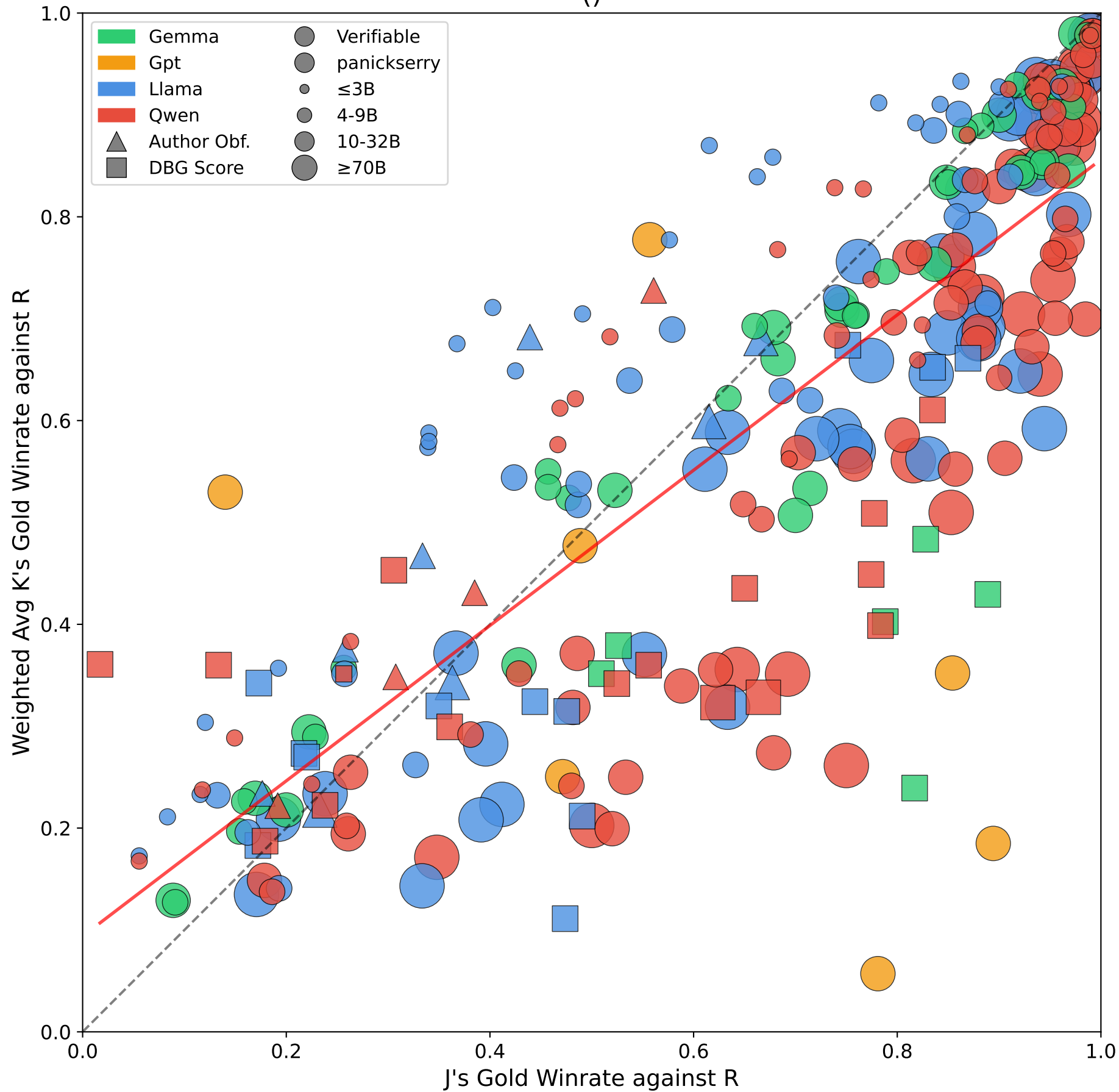
Gold Winrate Balance: J vs Weighted K ( )
