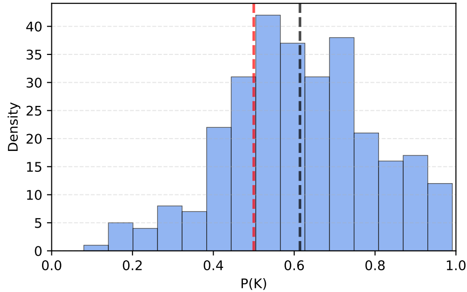
J(K vs R) - Combined \mu : 0.614 | Obj: 0.500 | n=292
