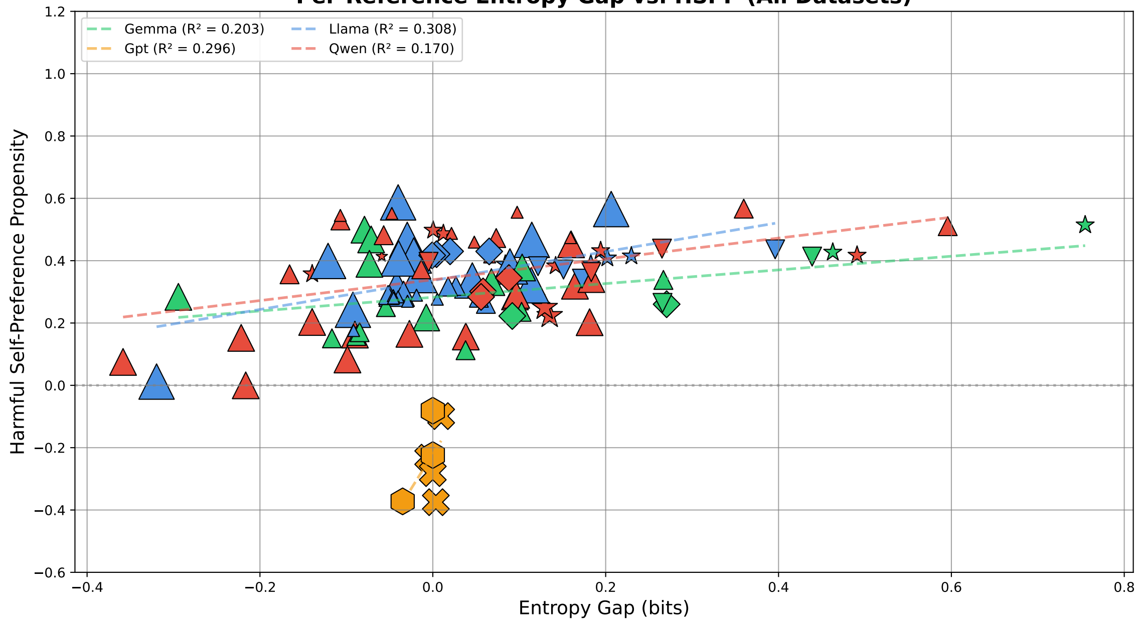
Per-Reference Entropy Gap vs. HSPP (All Datasets)
