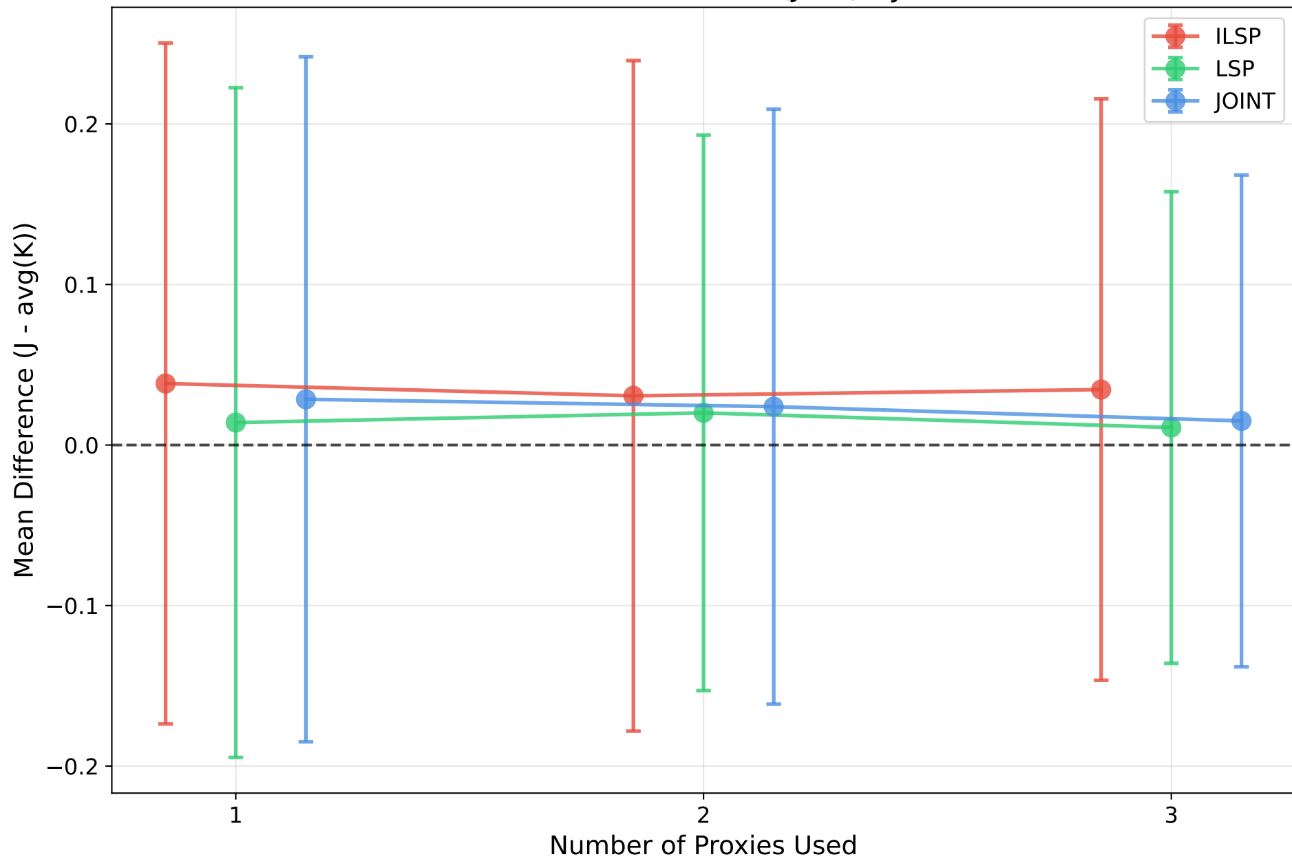
translation: Mean Difference (J - K) by # Proxies
