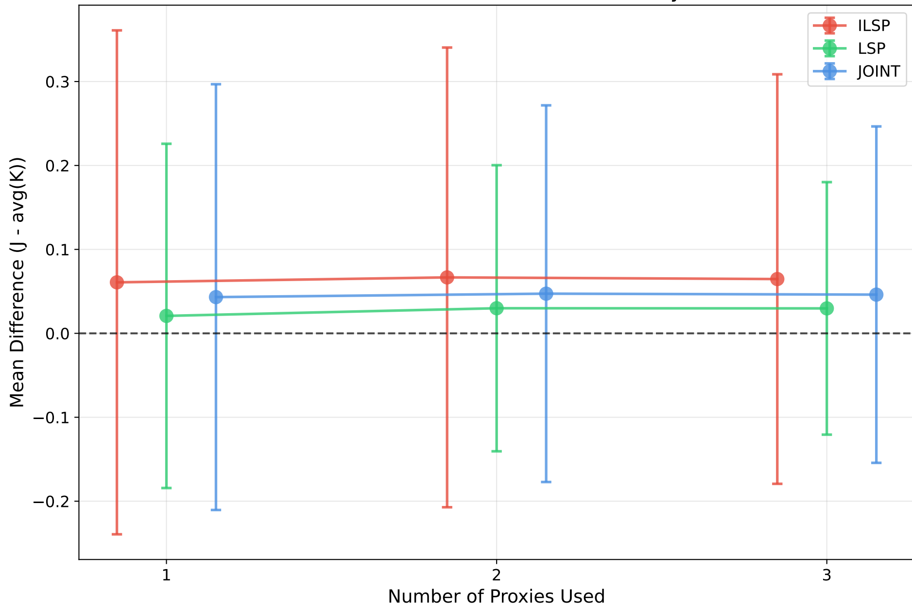
Llama-4-Scout-17B-16E-Instruct: Mean Diff by # Proxies
