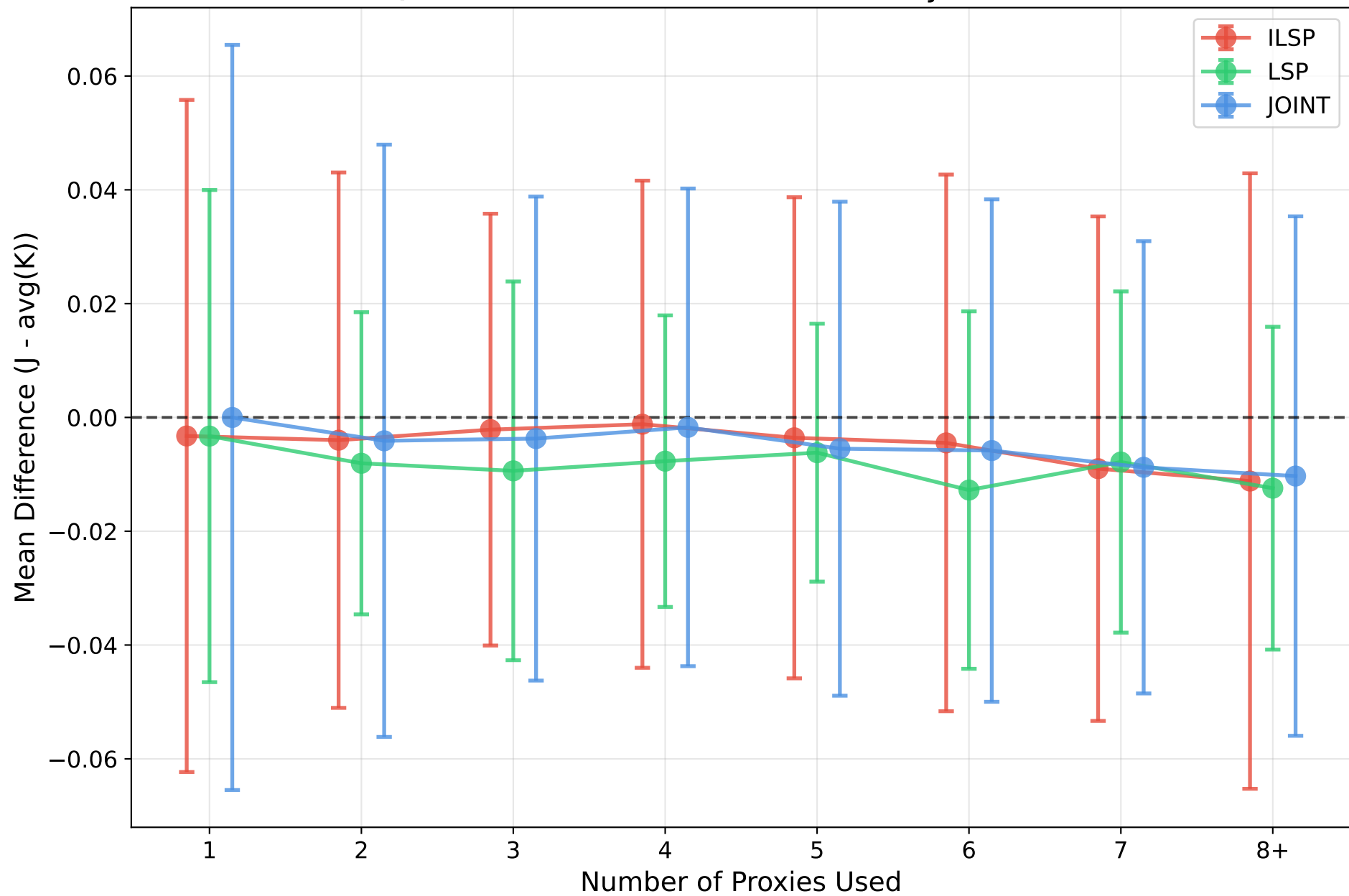
Qwen2.5-1.5B-Instruct: Mean Diff by # Proxies
