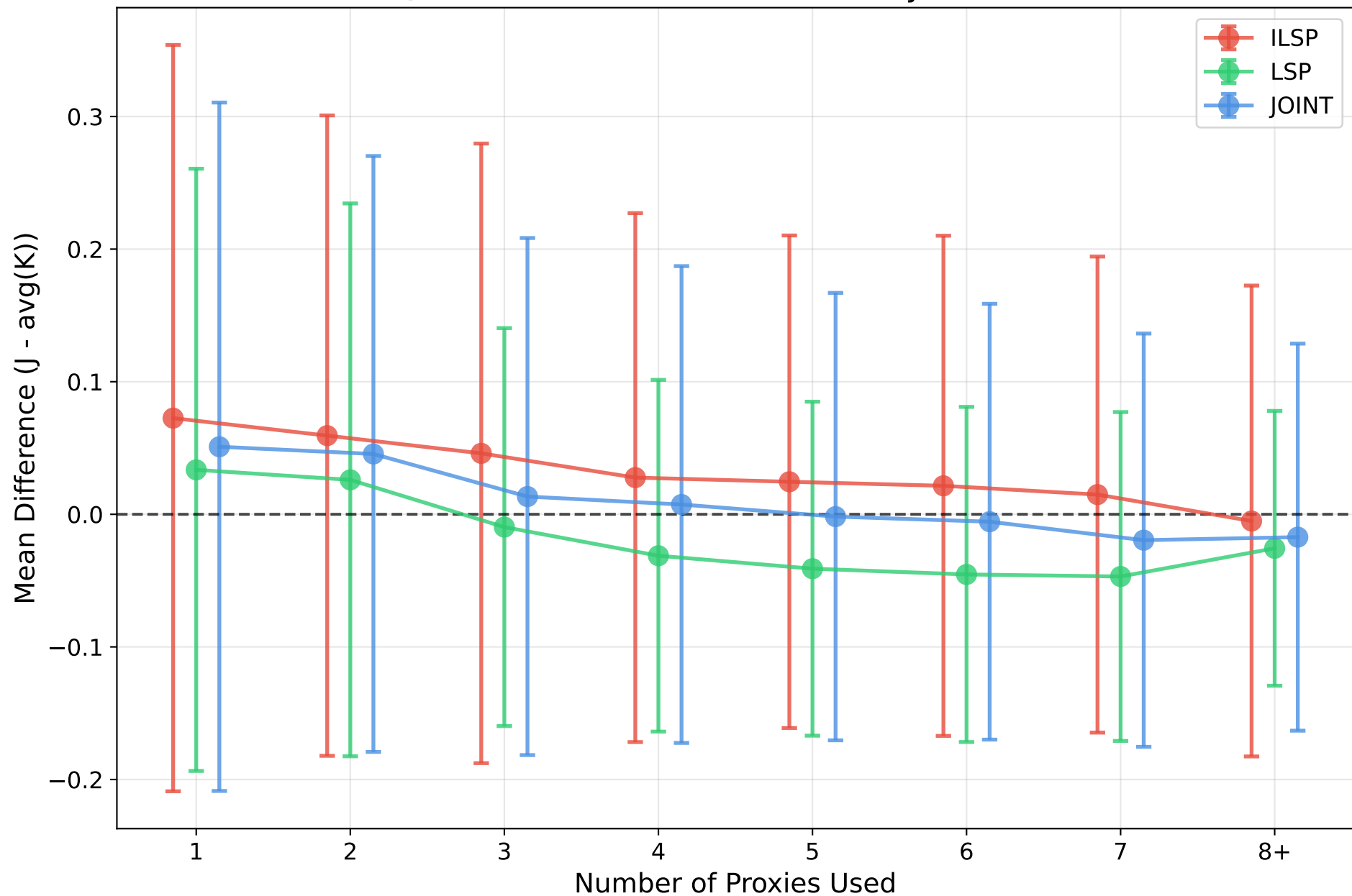
Qwen2.5-7B-Instruct: Mean Diff by # Proxies
