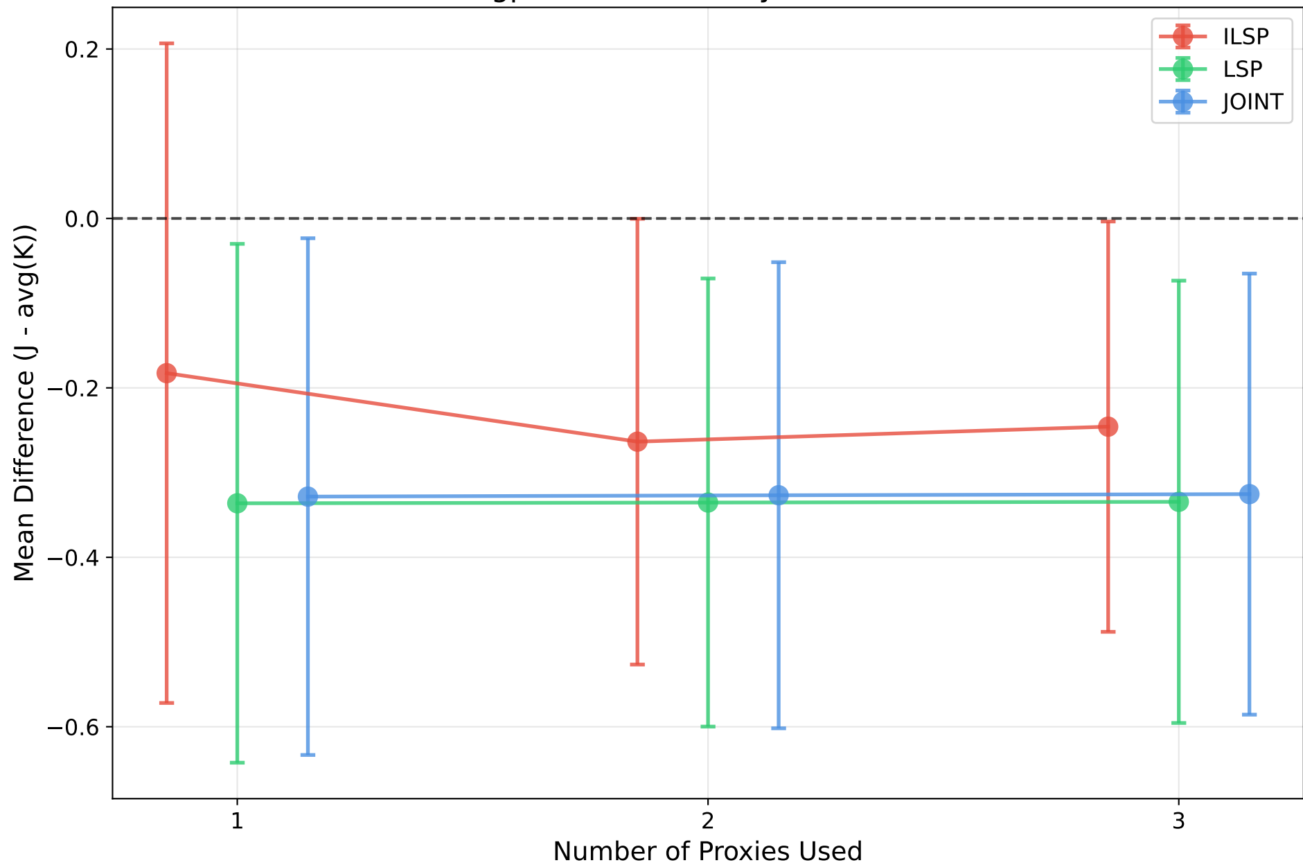
gpt-4: Mean Diff by # Proxies
