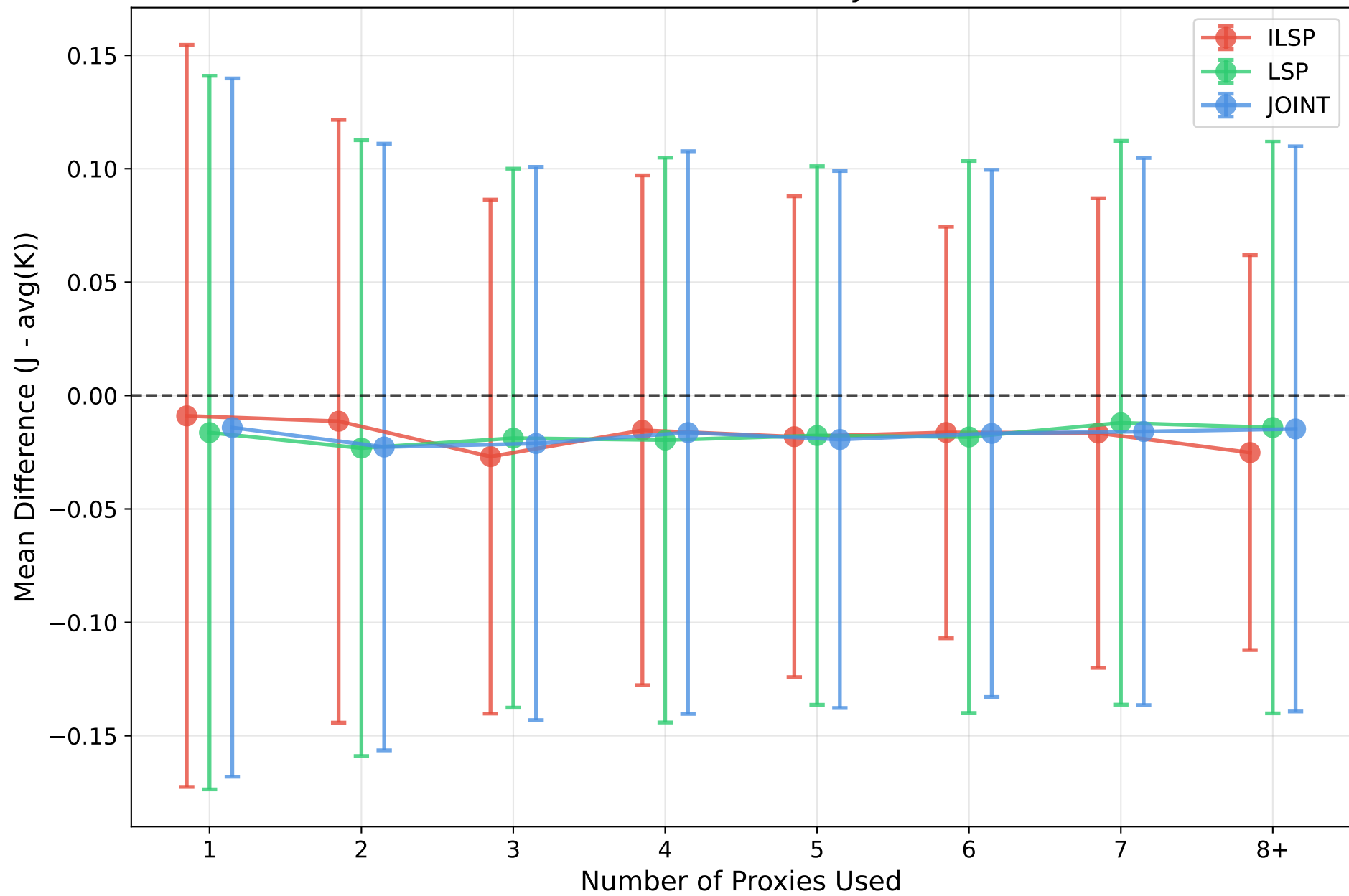
llama-3.1-8b: Mean Diff by # Proxies
