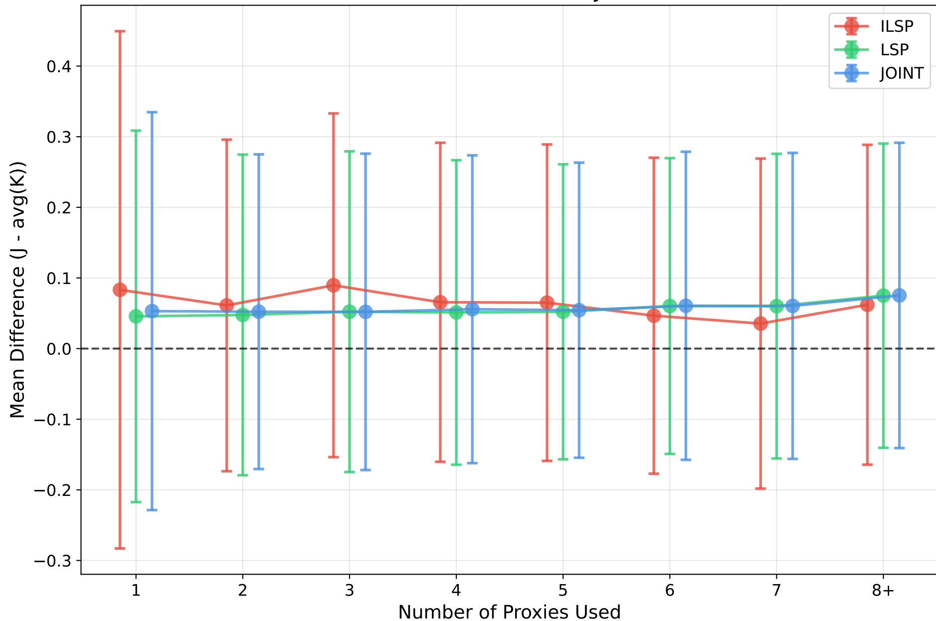
llama-3.3-70b: Mean Diff by # Proxies
