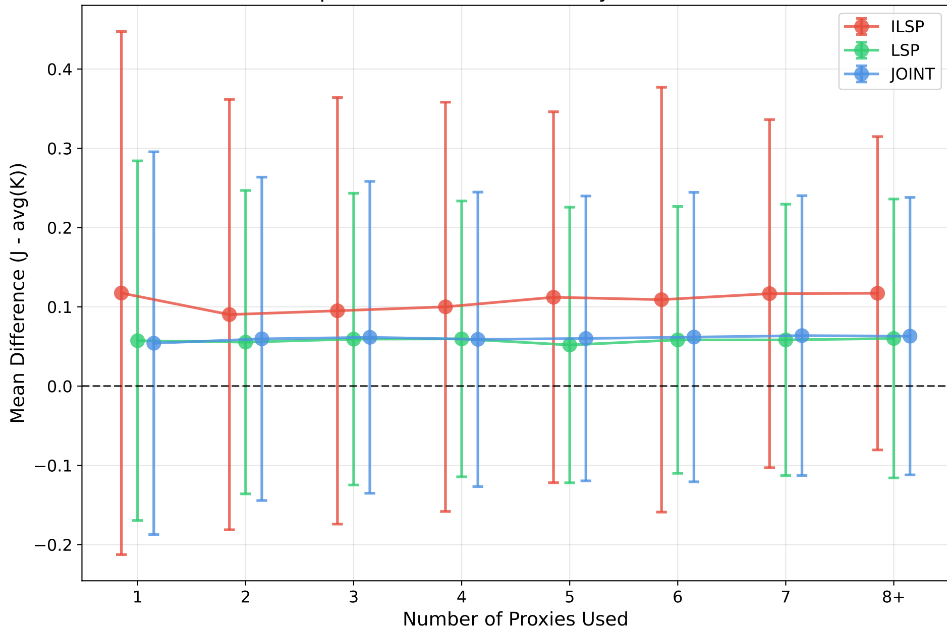
qwen-2.5-32b: Mean Diff by # Proxies
