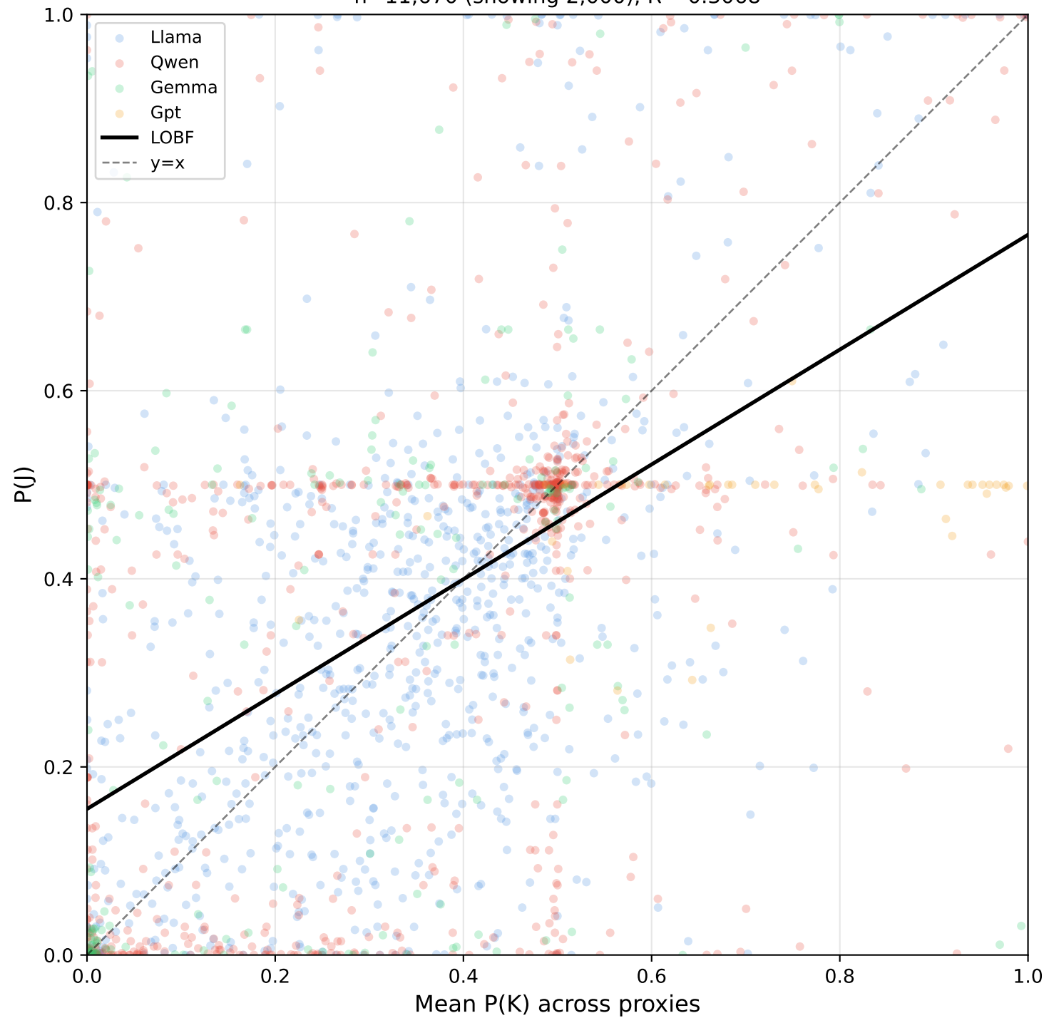
Per-Example: P(J|JvR) vs Mean P(K|KvR) n=11,670 (showing 2,000), R^2=0.3068
