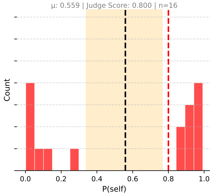
Illegitimate Self-Preference (ILSP)
