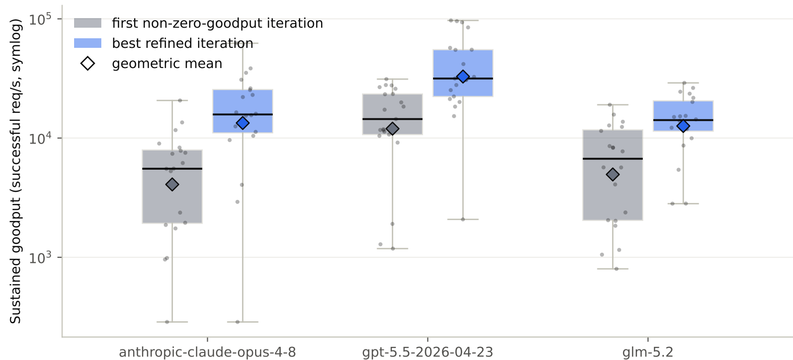
First-non-zero-goodput vs. best-refined goodput per model (box: quartiles and full range; diamond: geometric mean, as reported in the text; dots: individual scenario×framework cells)
