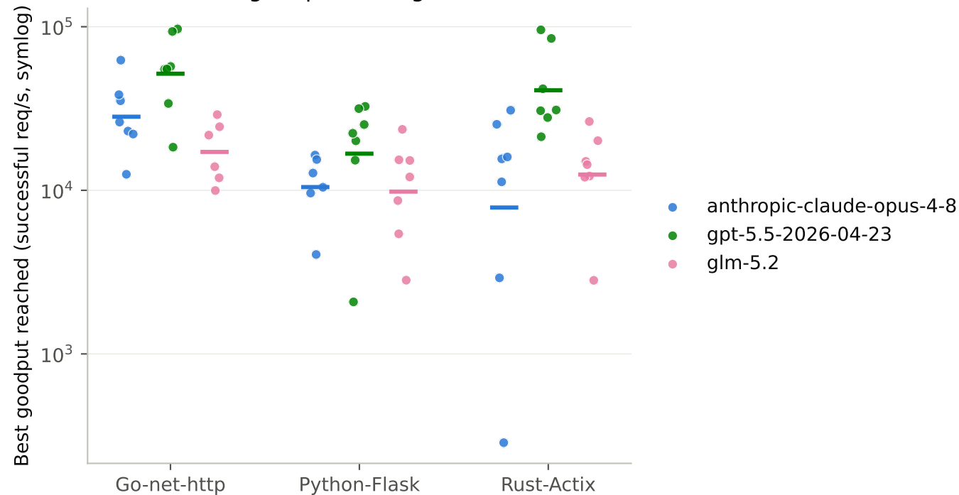
Best goodput reached per framework (dot: one scenario cell; bar: per-model geometric mean; cells with zero goodput throughout are excluded)
