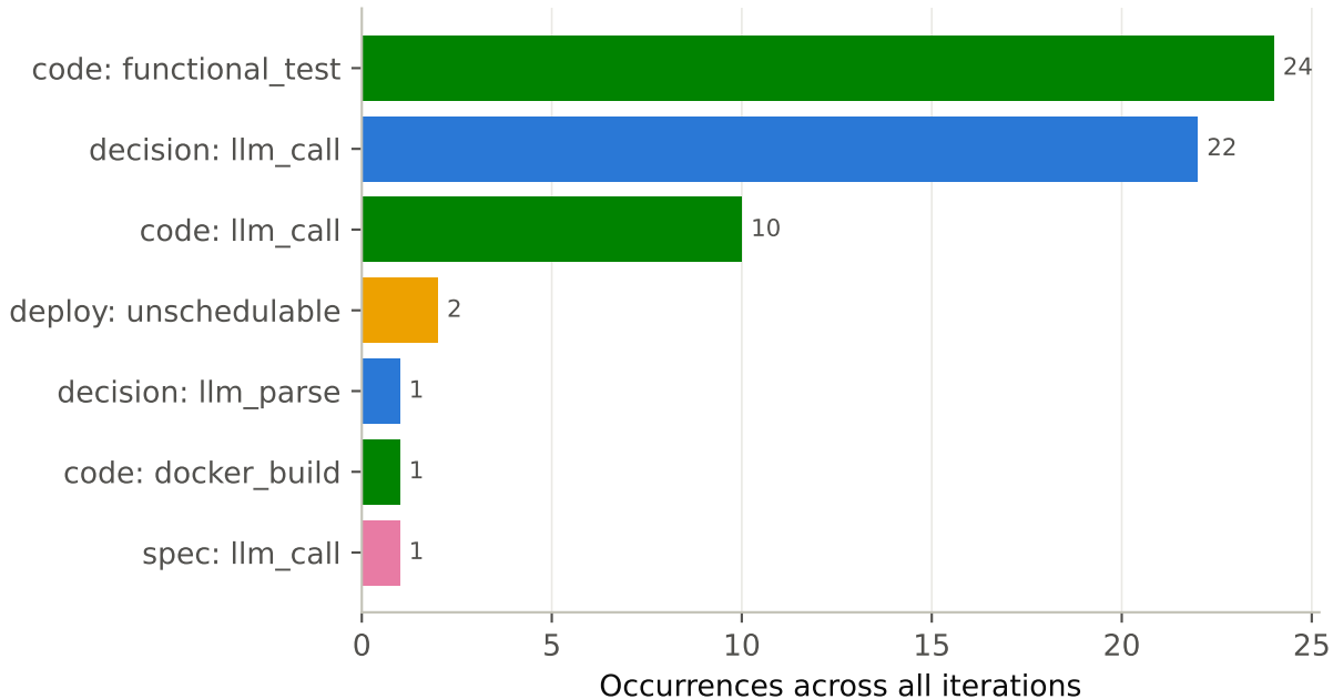
Top 7 failure kinds by phase
