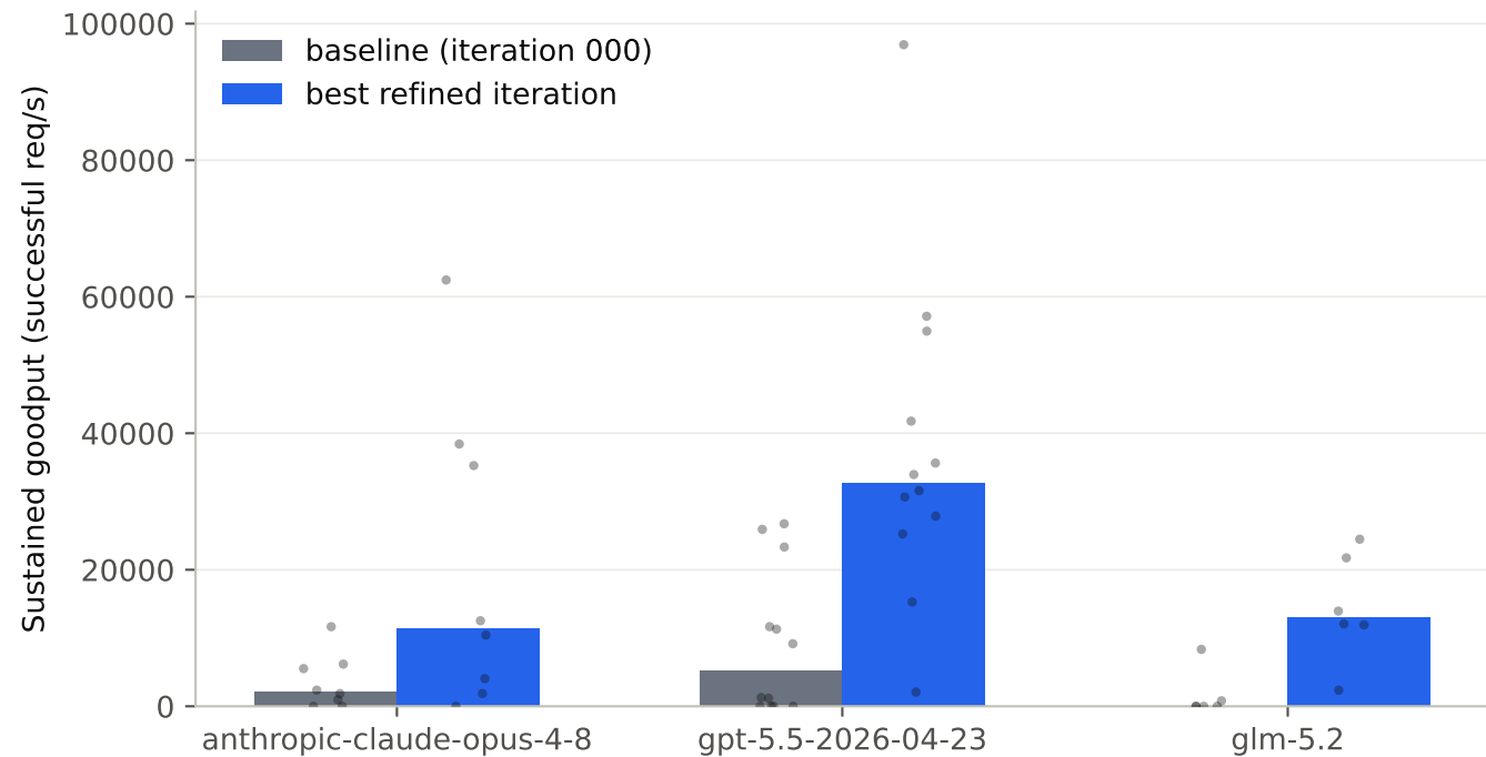
Median baseline vs. best-refined goodput per model (dots: individual scenario×framework cells)
