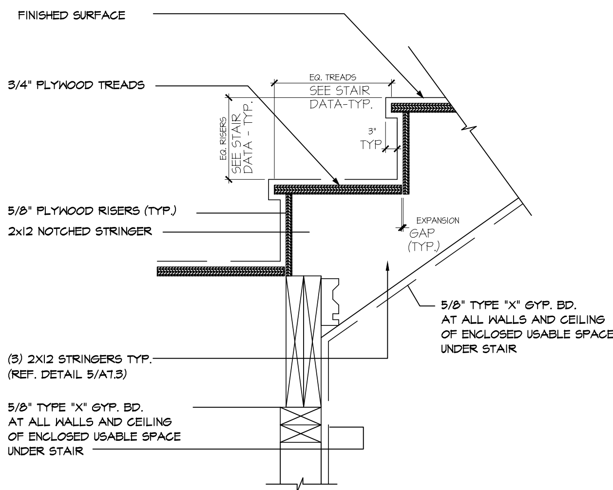
04 Landing/Stringer Detail SCALE: 1 1/2" = 1'-0" 02T06043.054_T4
