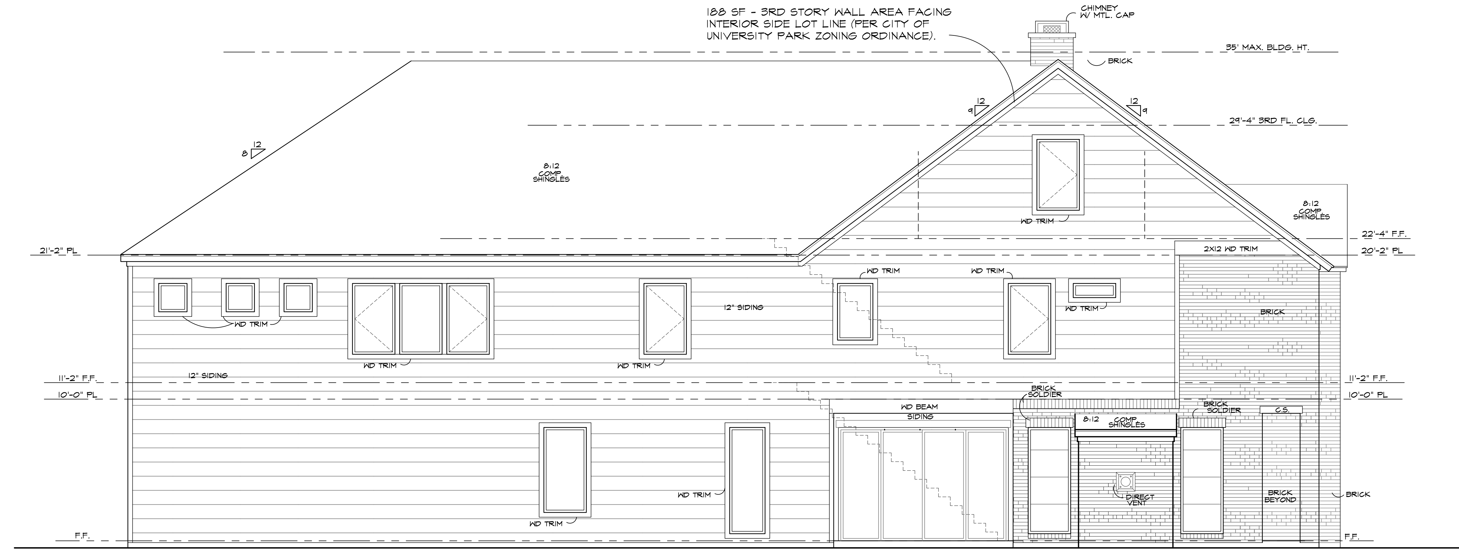
LEFT ELEVATION
