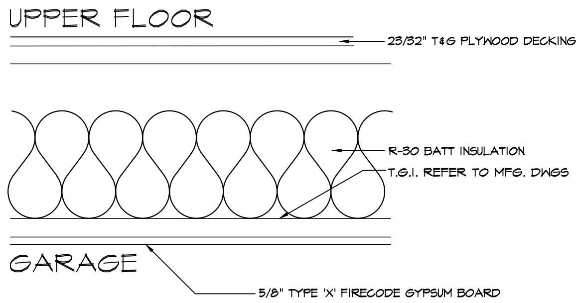
04 Typ. Mid Floor With Insulation SCALE: 1/2" = 1'-0"
