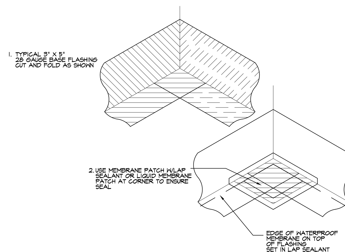
07 Flashing Detail at Inside Cnr. SCALE: 3" = 1'-0"
