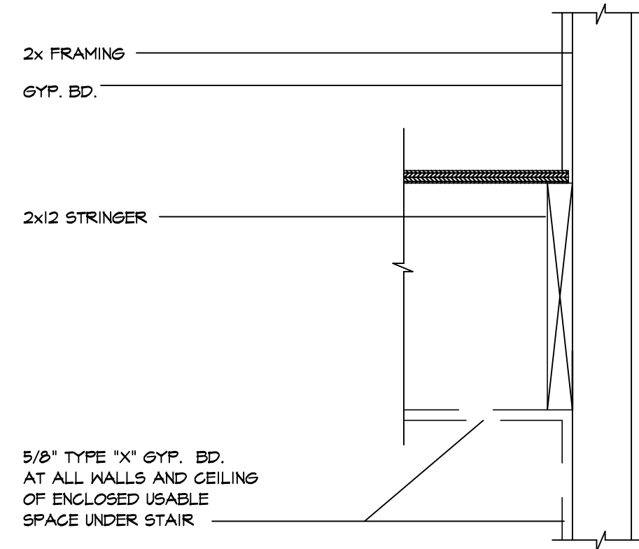
02 Stringer/Wall Detail SCALE: 1 1/2" = 1'-0" 02T06043.054_T6
