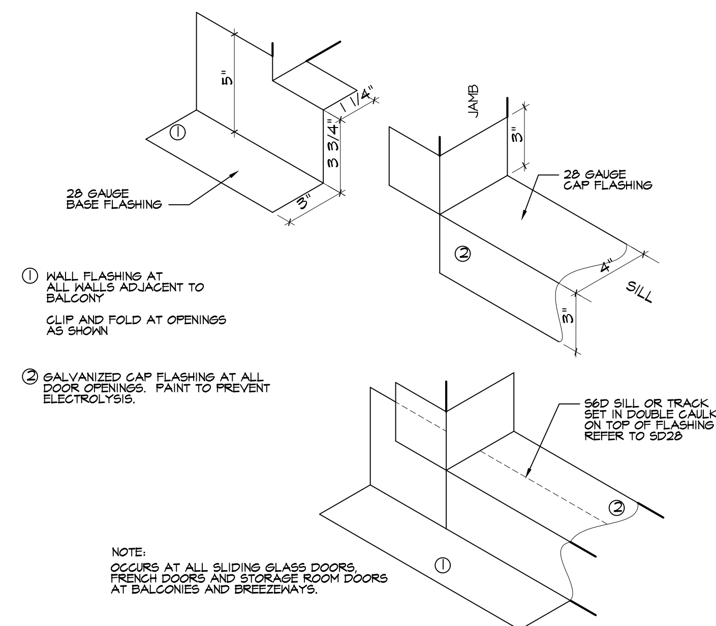
Flash'g at Door Openings
