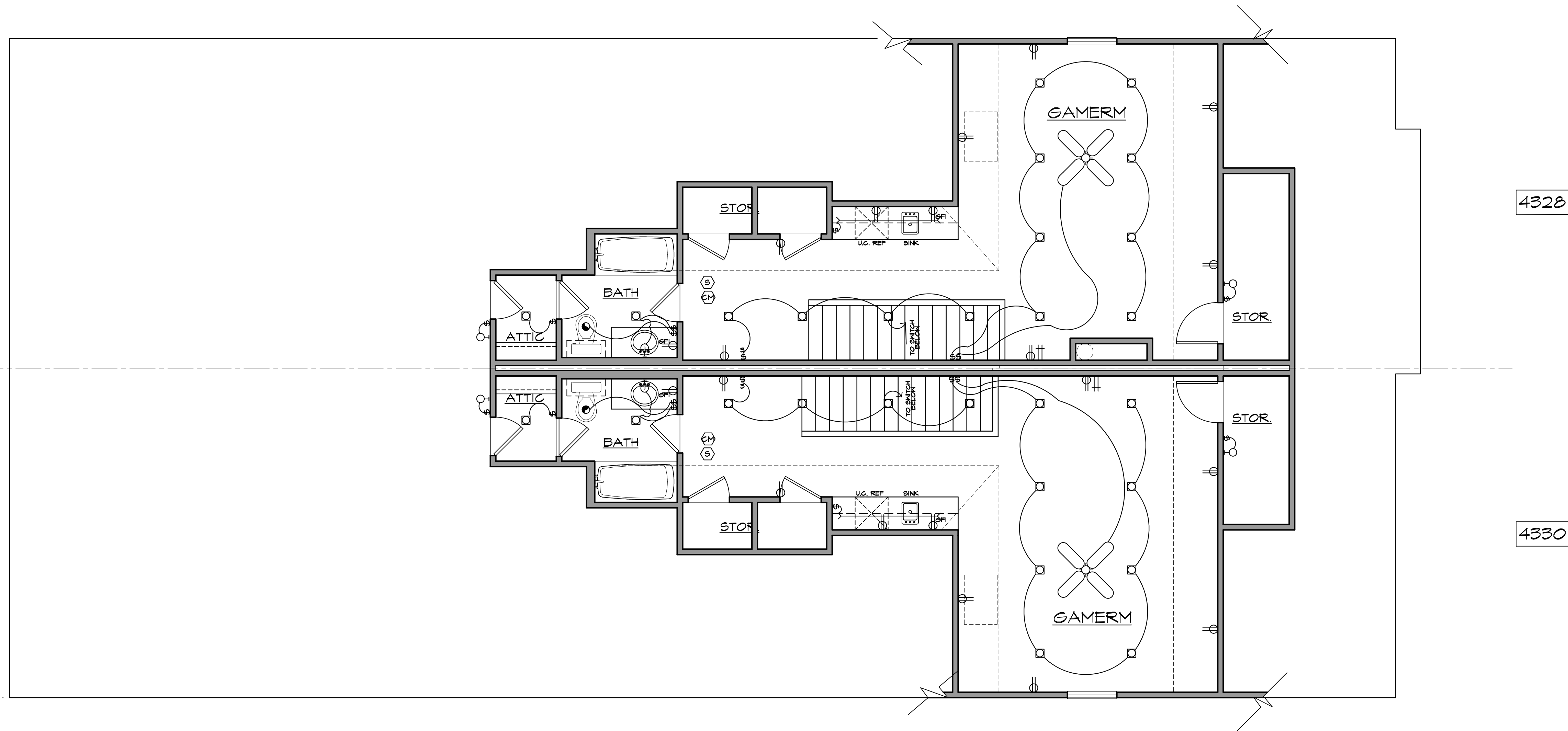
THIRD FLOOR ELECTRICAL PLAN
