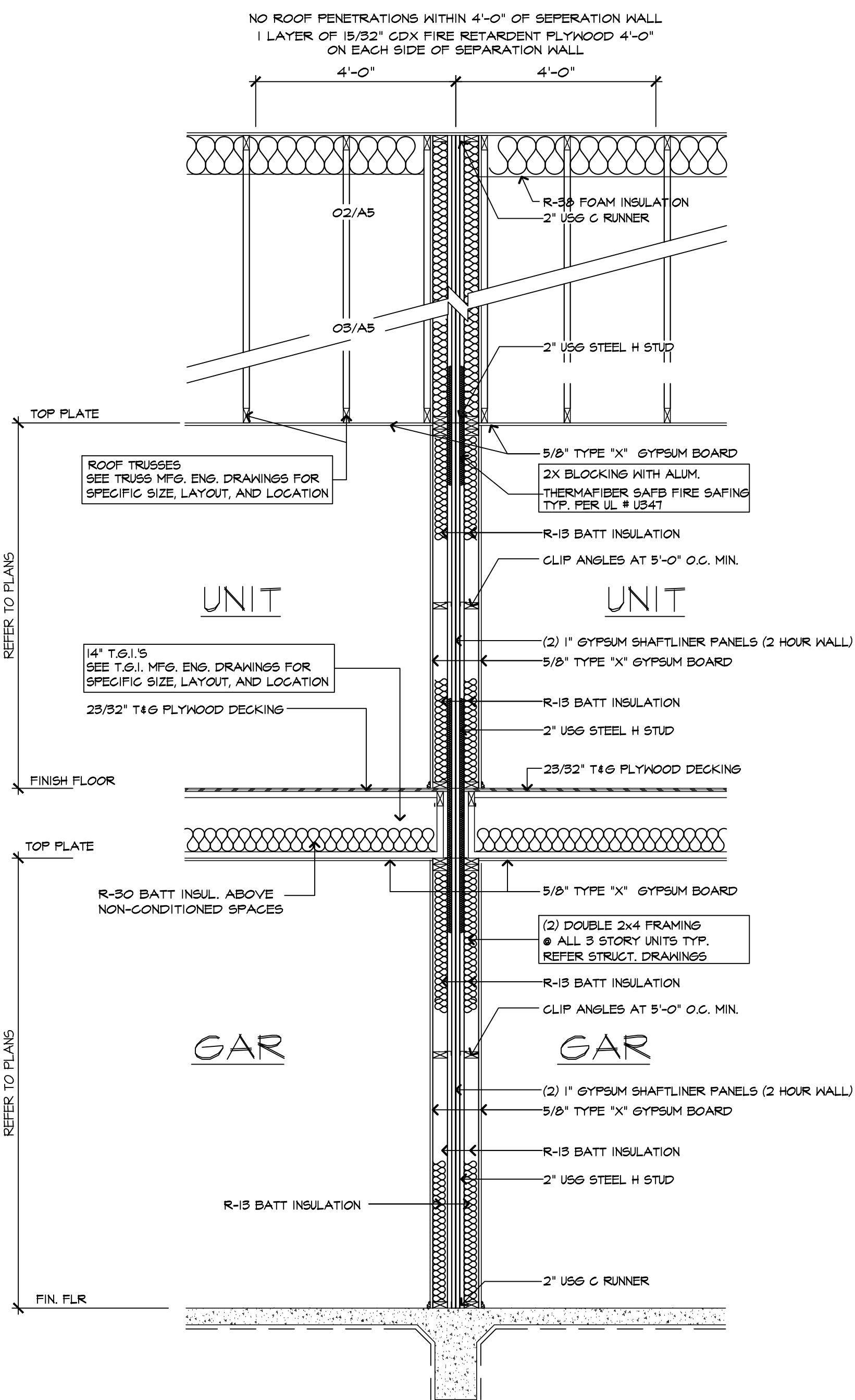
02 Typ. Party Wall Section SCALE: 1/2" = 1'-0" 2 HOUR RATING PER UL # U347 CONFIG B: STC 70
