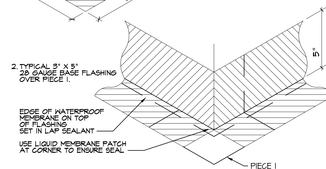
08 Flashing Detail at Outside Crnr. SCALE: 3" = 1'-0"
