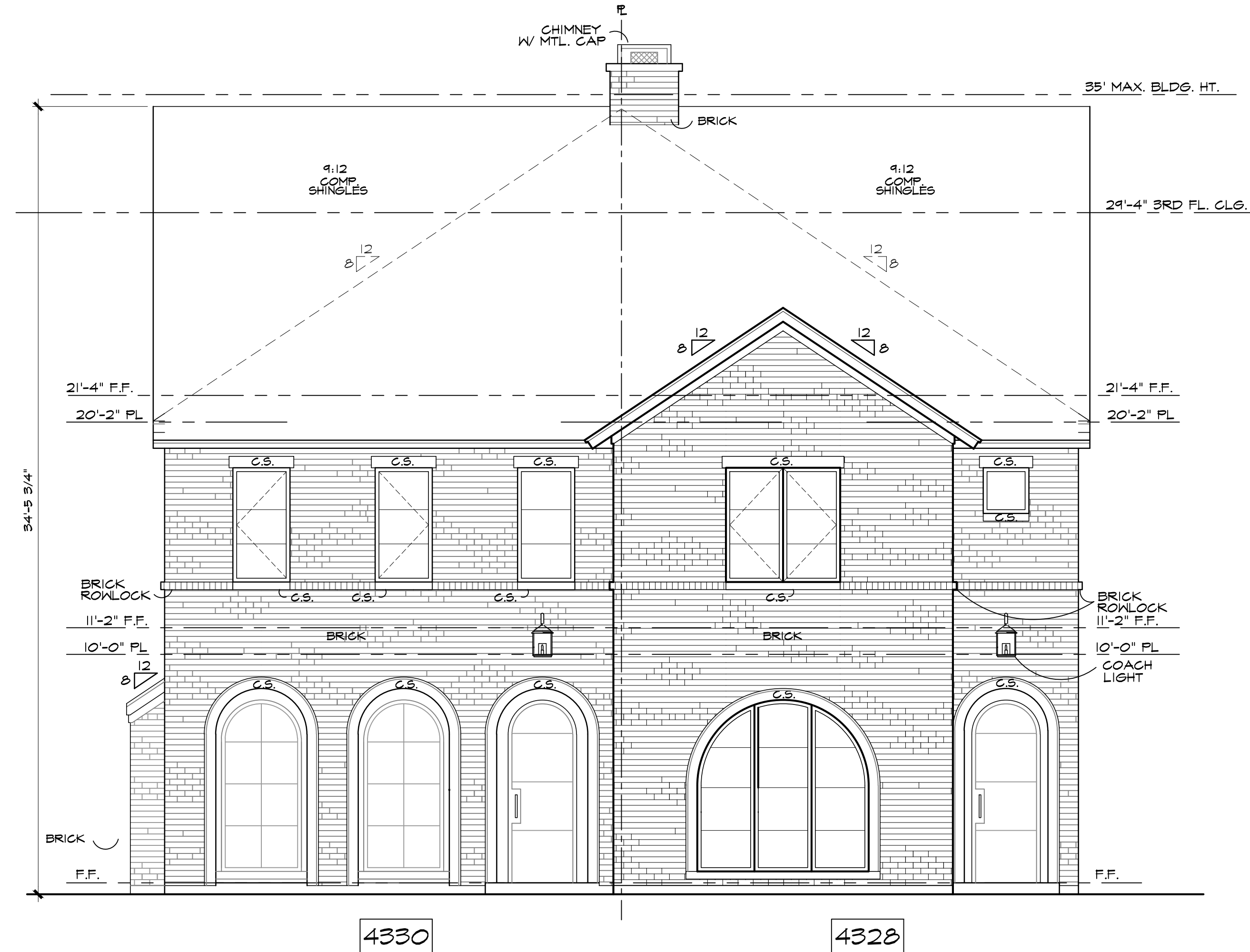
FRONT ELEVATION
