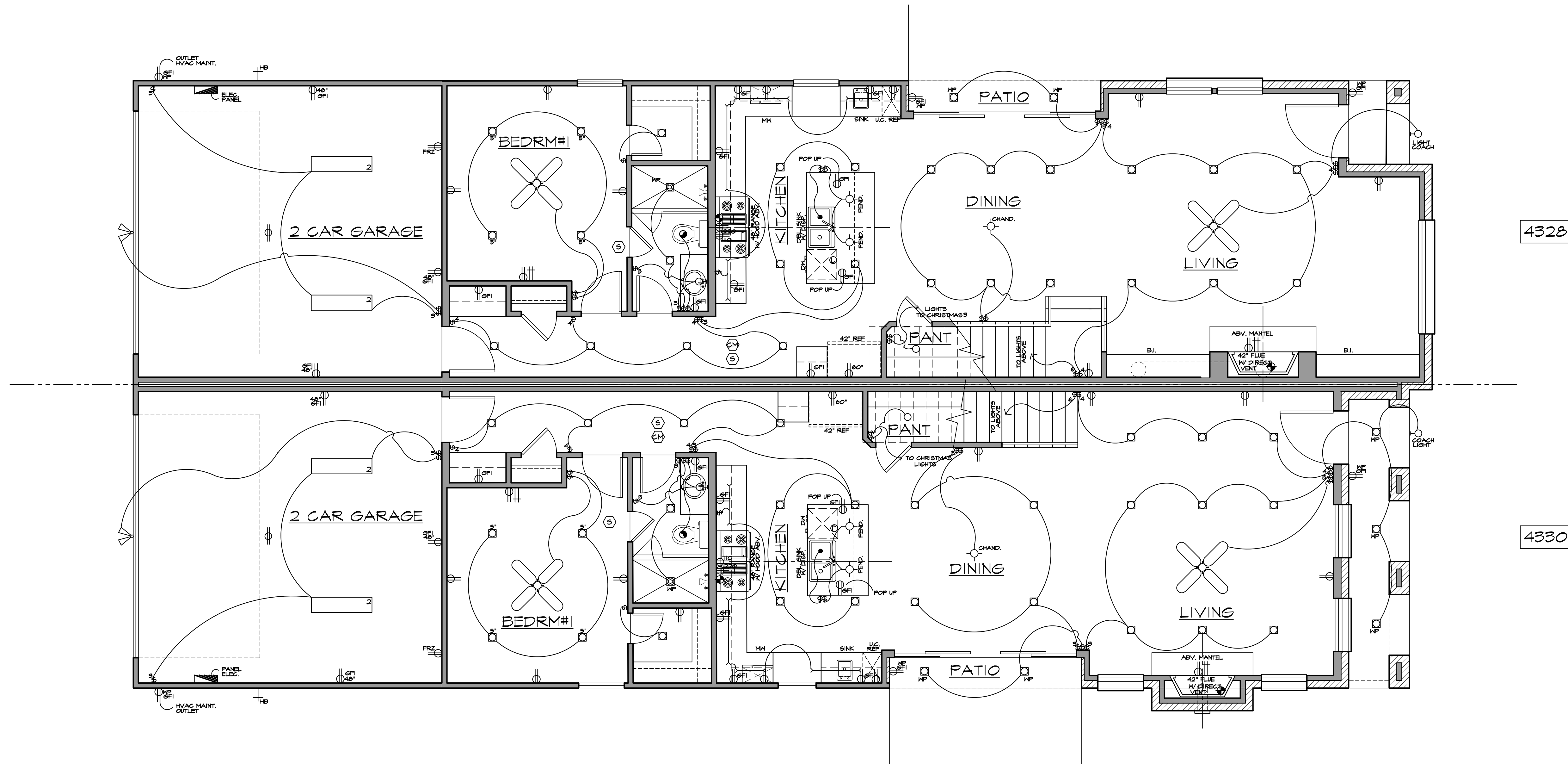
FIRST FLOOR ELECTRICAL PLAN
