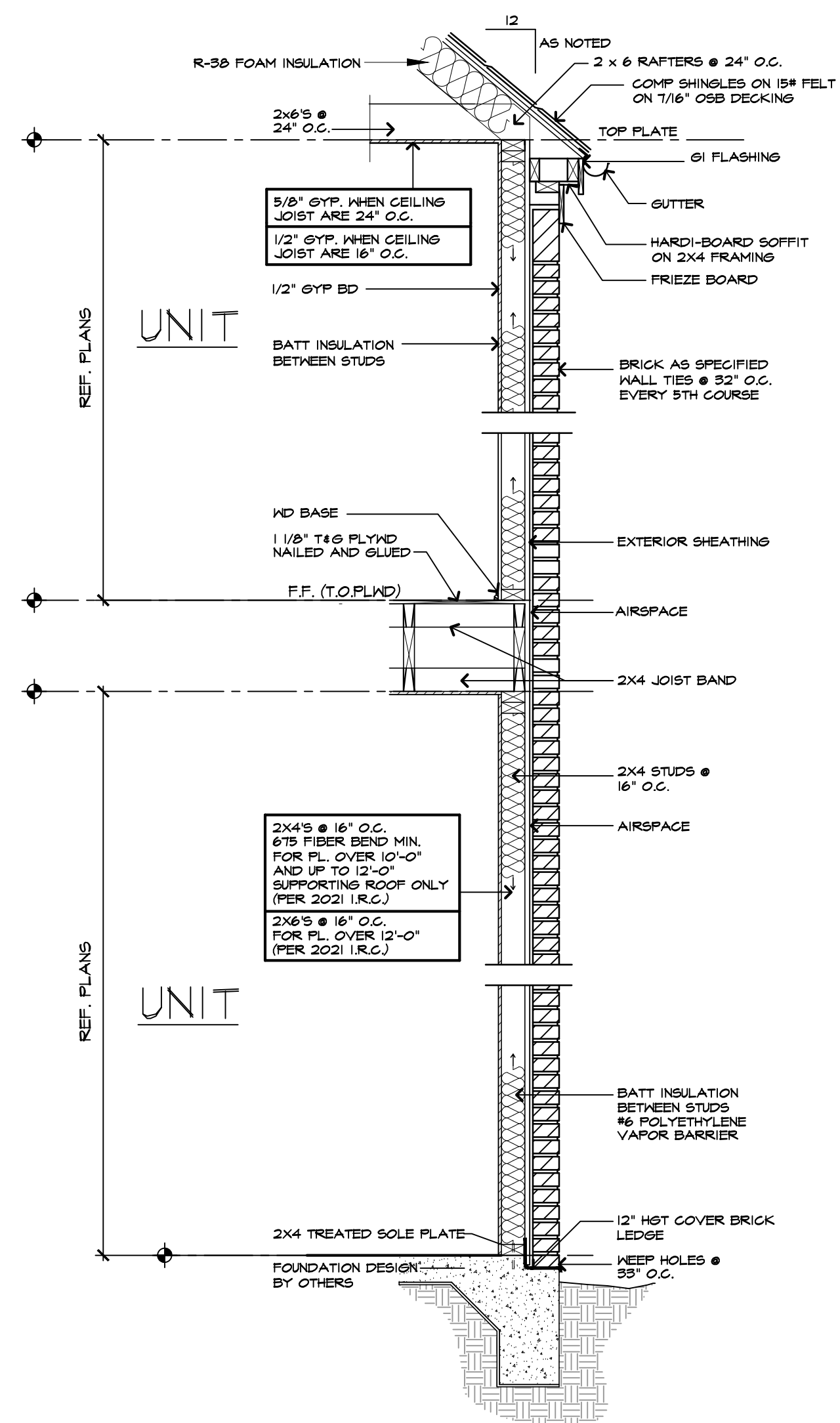
01 Typ. Exterior Wall Section SCALE: 1/2" = 1'-0"
