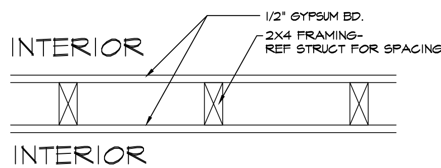
08 Typ. Interior Wall SCALE: 1/2" = 1'-0"
