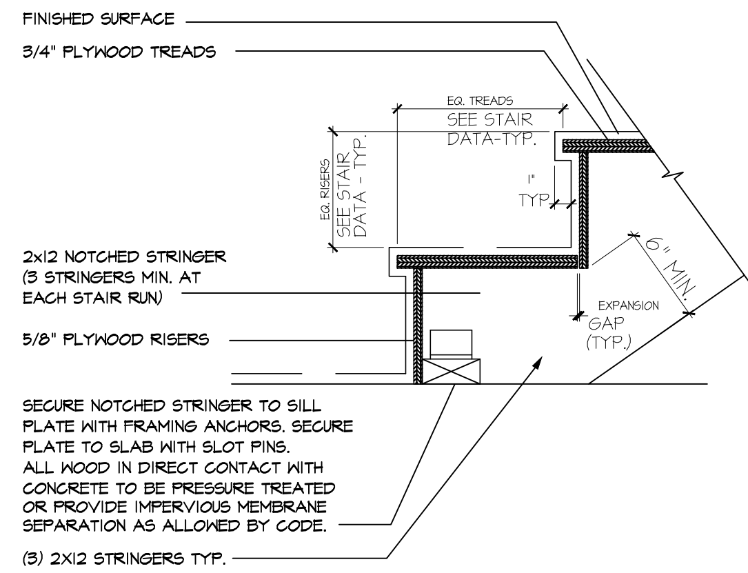
03 Floor/Stringer Detail SCALE: 1 1/2" = 1'-0" 02T06043.054_T5
