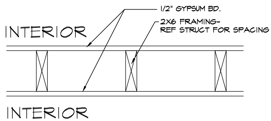
07 Typ. Interior Wall SCALE: 1/2" = 1'-0"
