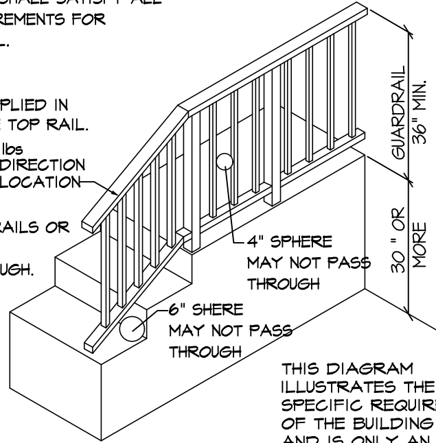
06 Handrail/Guardrail Code Data SCALE: 1 1/2" = 1'-0" 02T06043.054_T2
