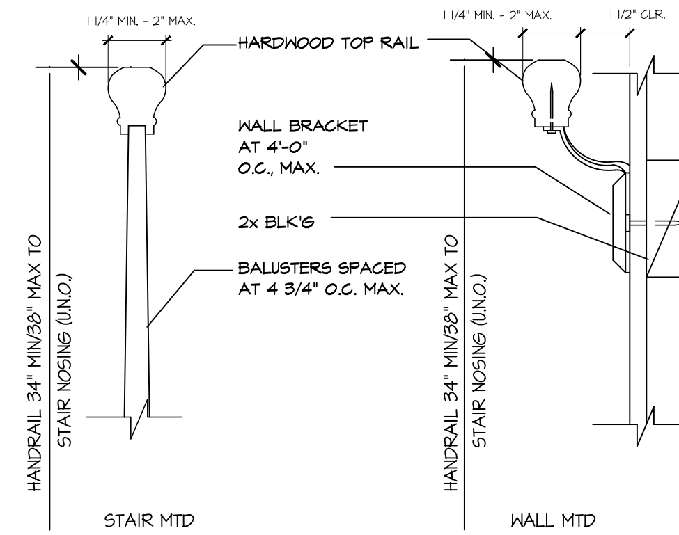
01 Handrail Detail SCALE: 1 1/2" = 1'-0" 02T06043.054_T7
