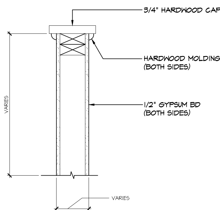
07 Typ. Low Wall Detail SCALE: 1 1/2" = 1'-0"
