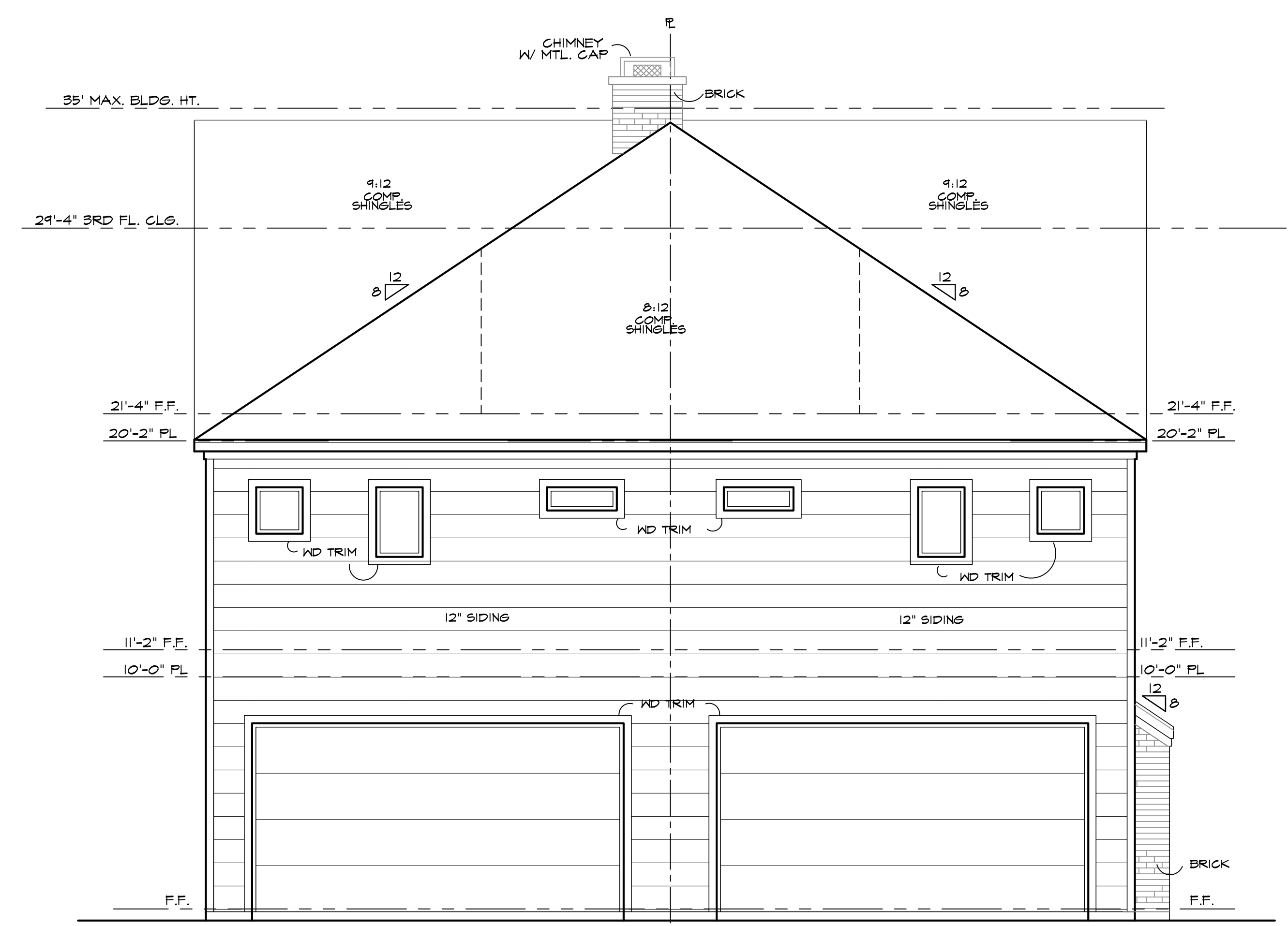
REAR ELEVATION
