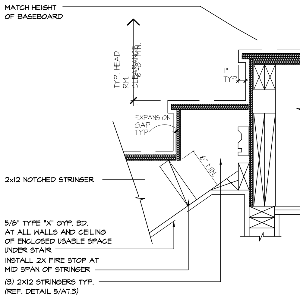
05 Stringer/Landing Detail SCALE: 1 1/2" = 1'-0" 02T06043.054_T3
