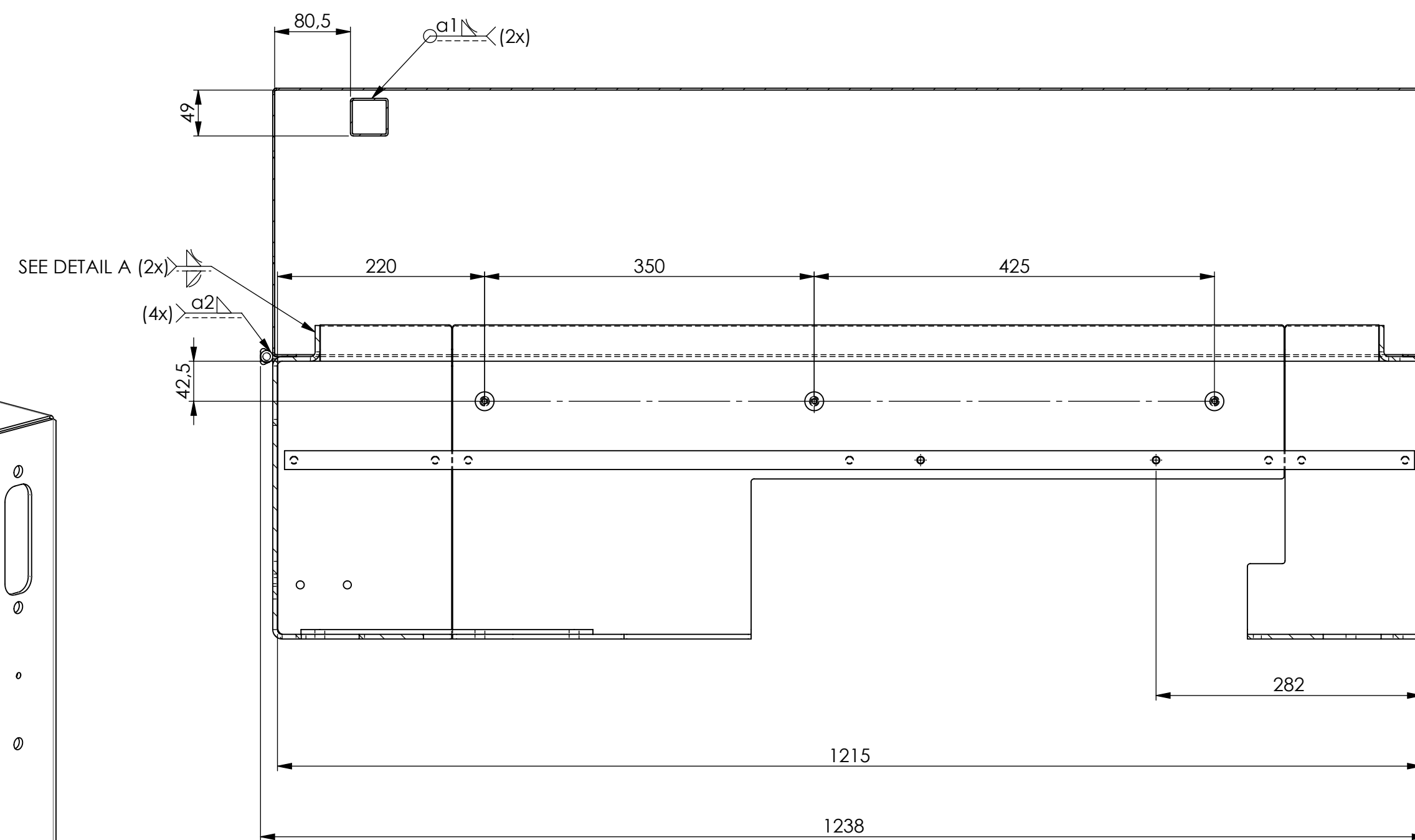
SECTION B-B
