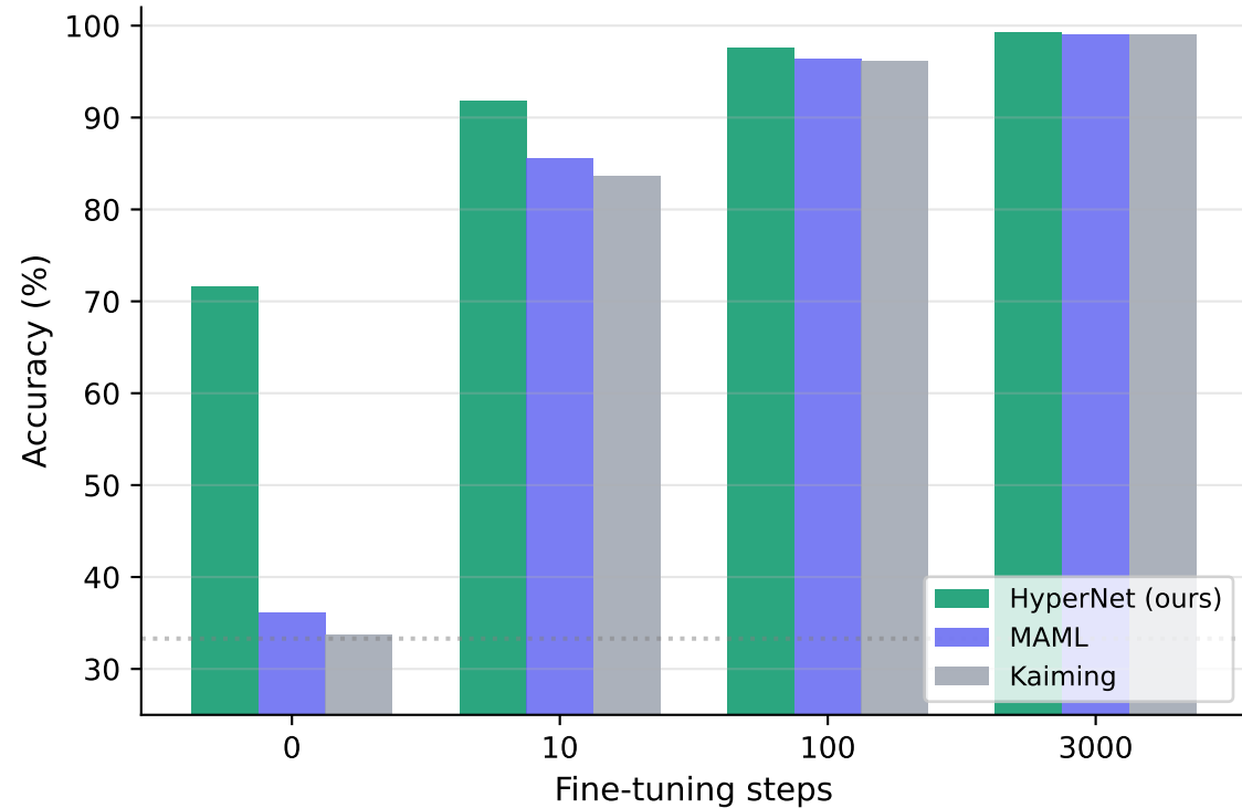
HyperNet vs MAML vs Kaiming (digits-unseen, trained on letters only)
