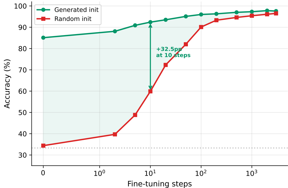
Convergence: Generated vs Random (50 unseen-digit tasks, mean)
