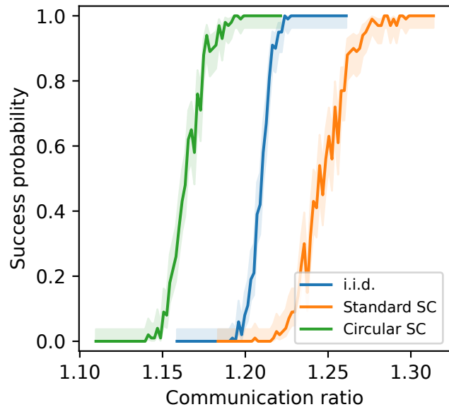
k=2, \text{ell}=3
