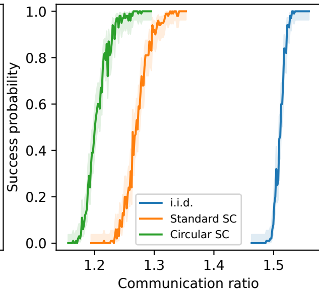
k=3, \text{ell}=4
