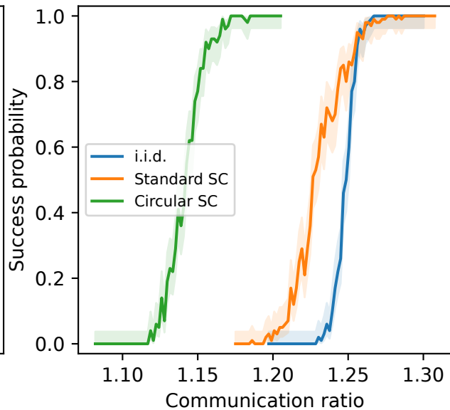
k=2, \text{ell}=6
