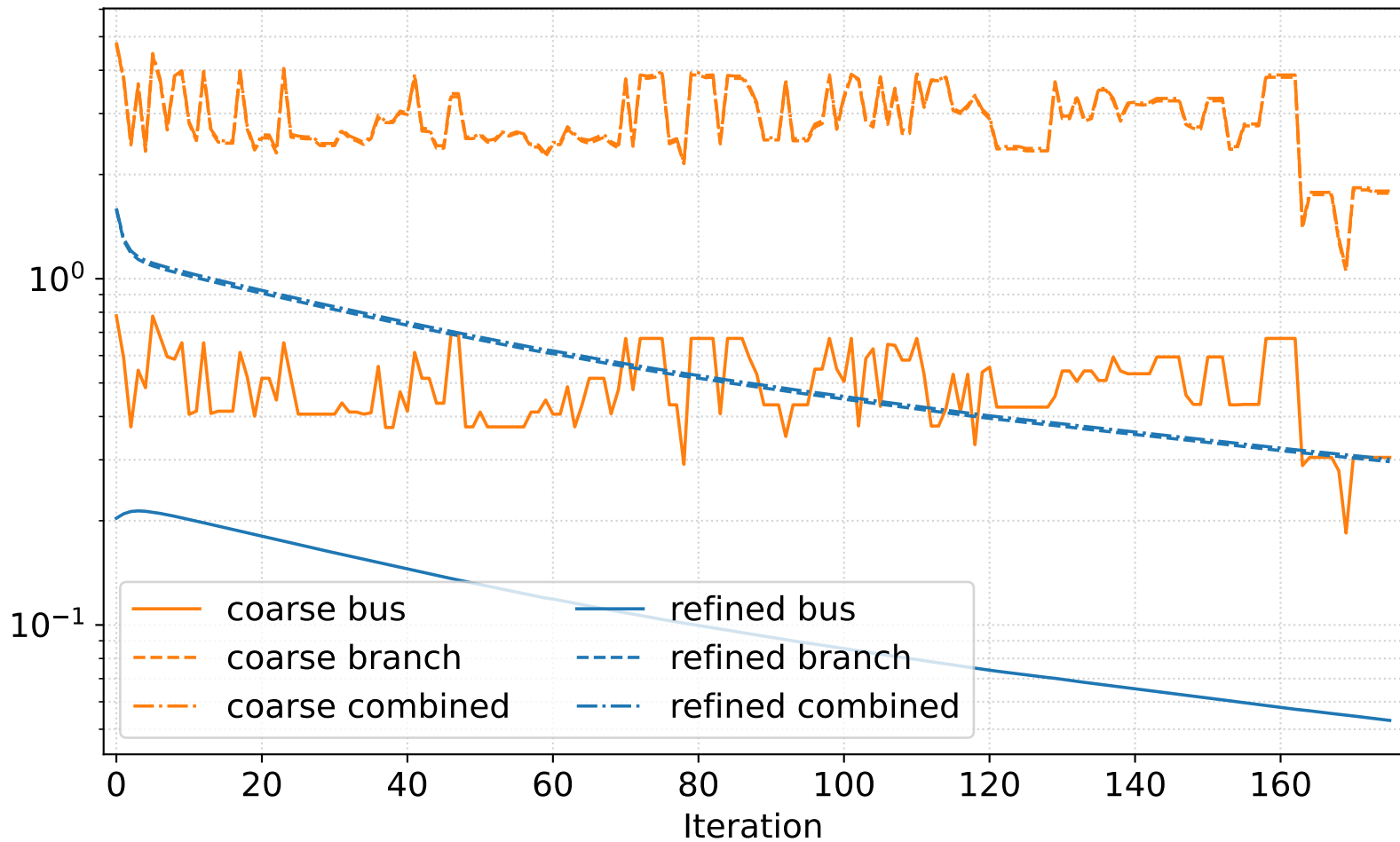
Euclidean distance
