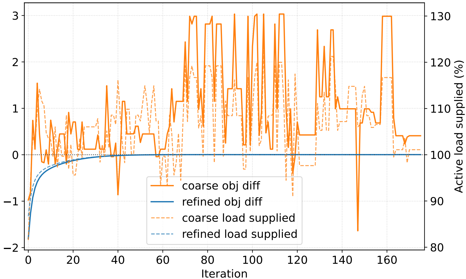
Objective difference
