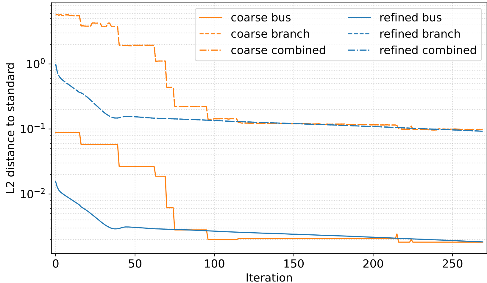
Euclidean distance
