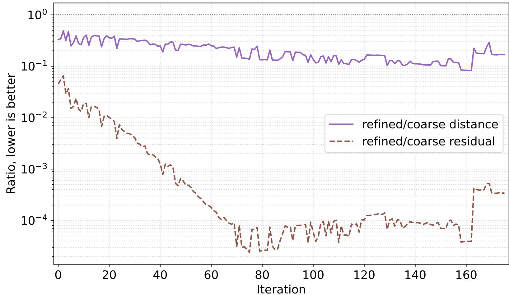
Refinement contraction
