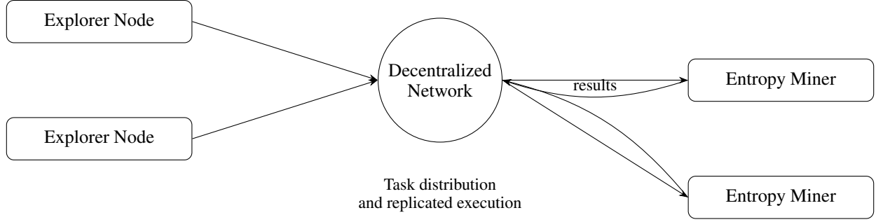
Figure 1: Logical architecture of the Doomsday Explorer framework. Explorer Nodes define computational experiments. The decentralized verification network distributes workloads, selectively replicates tasks, aggregates returned observations, and publishes reproducible evidence. Independent replication mitigates result withholding and enables verification of published computational results.
