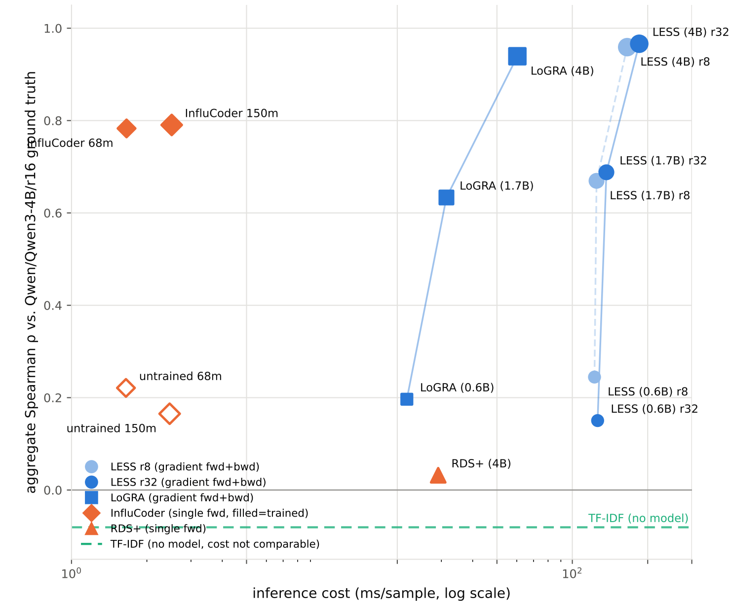
EXP1 Part 1 (BIG_GPU_FINAL) — 800x800 eval LESS r=8/32 (every size, both ranks), LoGRA r=32 (uniform, batched)
