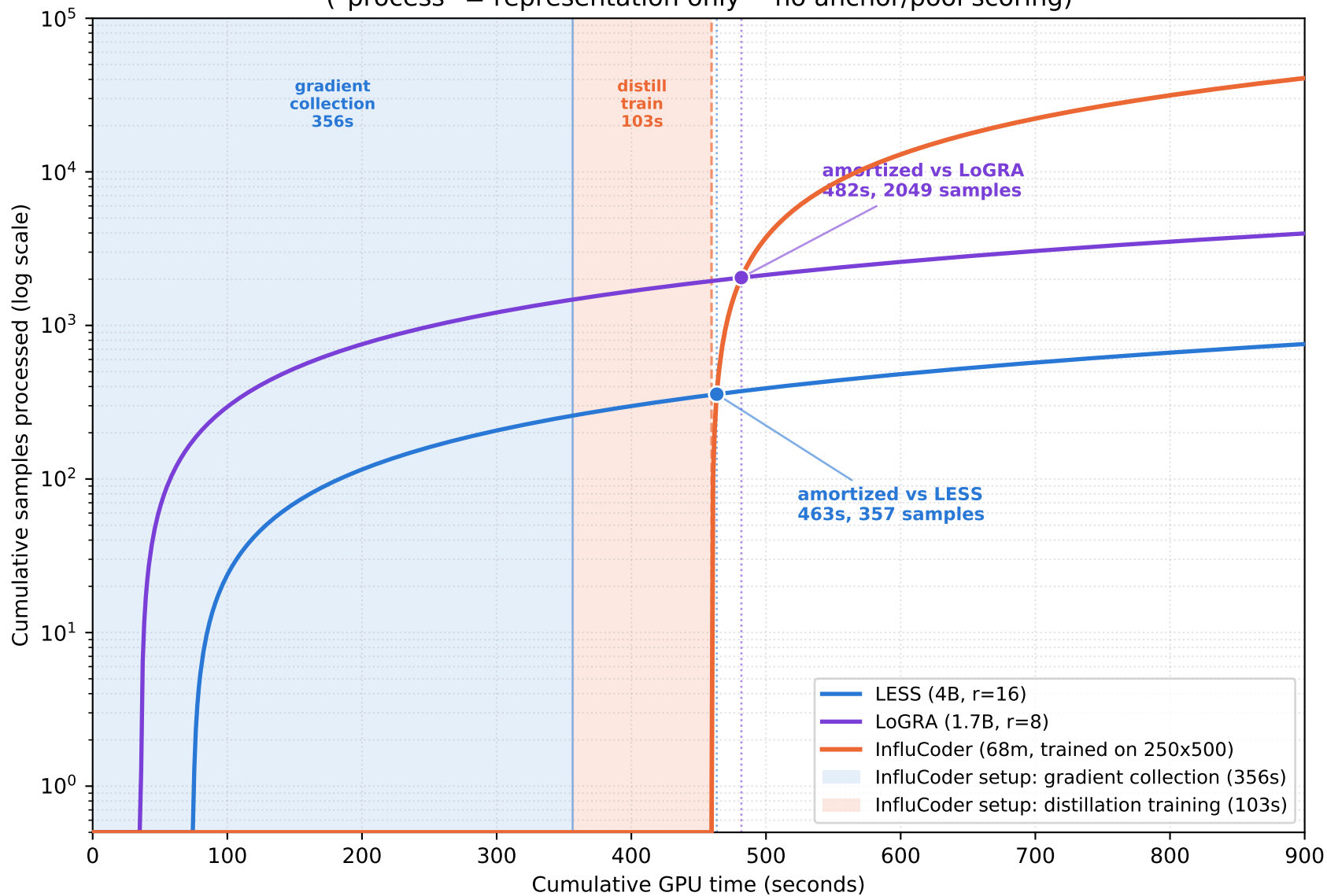
EXP1 Figure 1, Part 3: GPU-time-vs-samples-processed ("process" = representation only -- no anchor/pool scoring)
