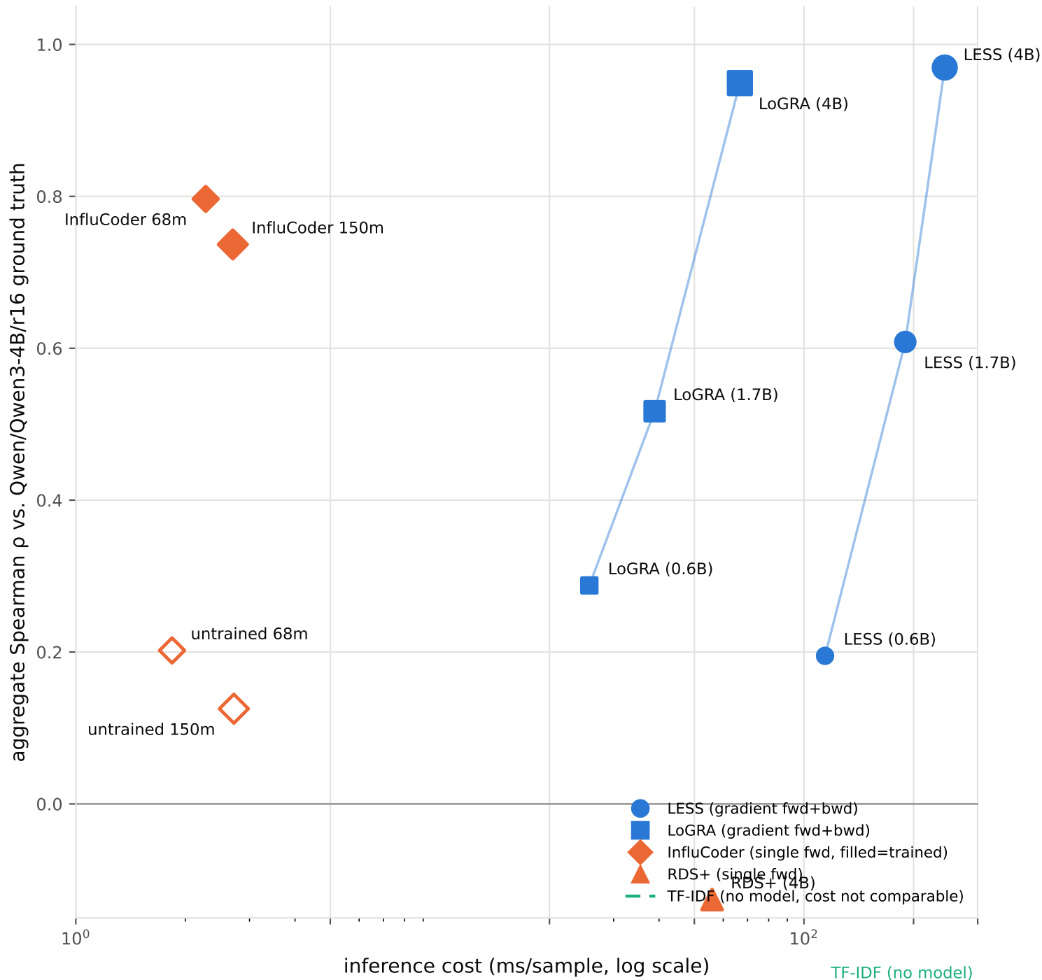
EXP1 Part 1 (BIG_GPU_FINAL) — 50x50 eval LESS r=32, LoGRA r=32 (uniform, batched)
