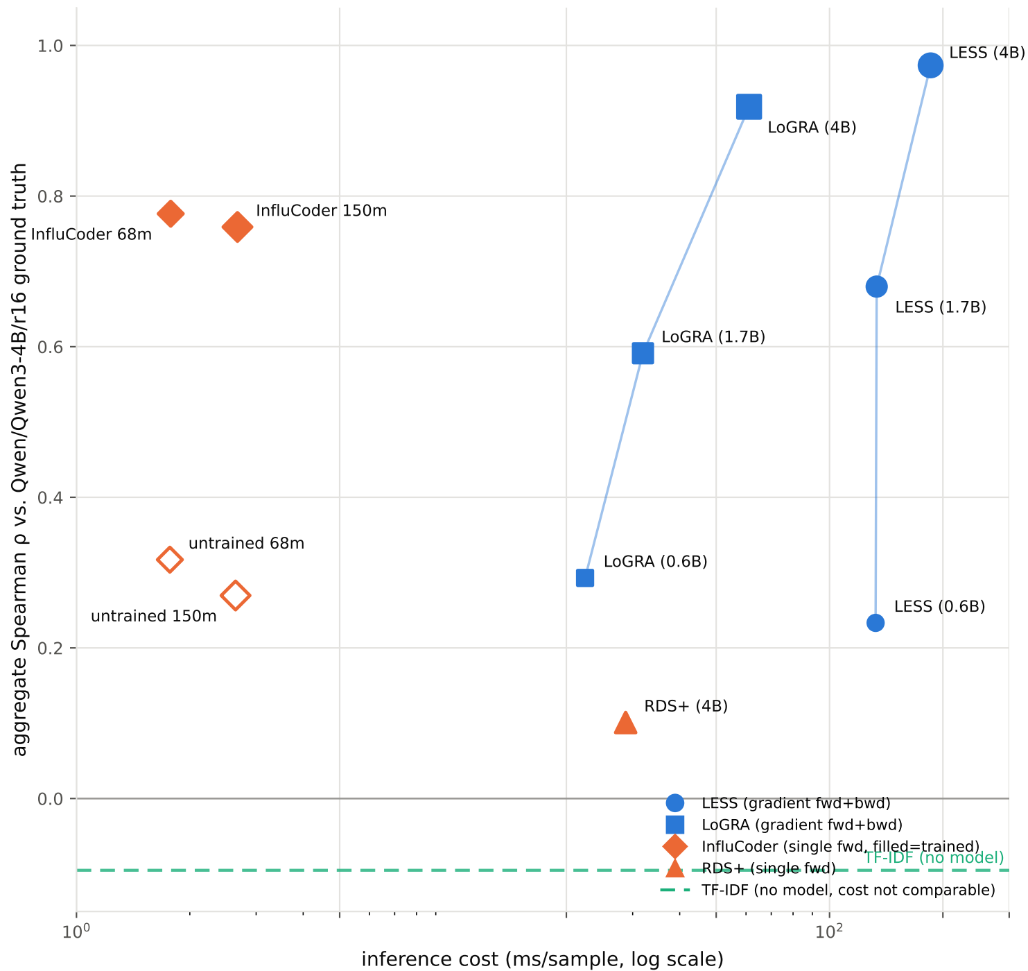
EXP1 Part 1 (BIG_GPU_FINAL) — 400x400 eval LESS r=32, LoGRA r=32 (uniform, batched)
