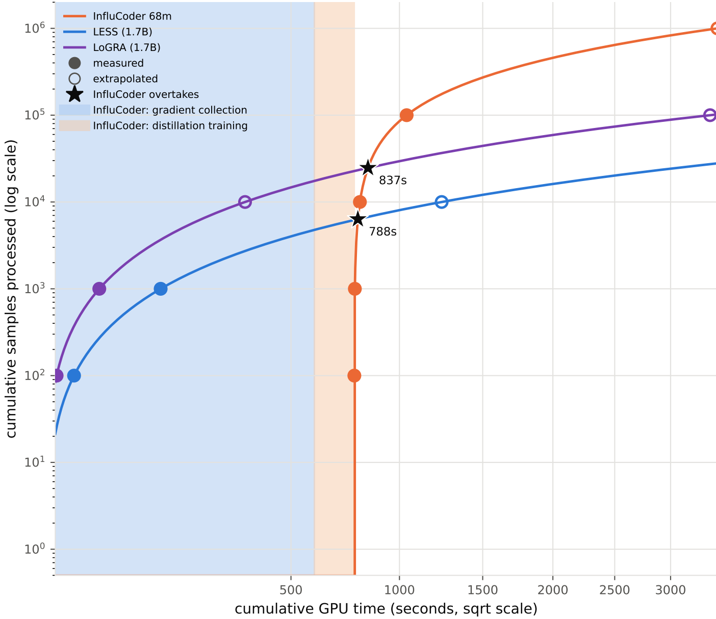
EXP1 Part 3 (BIG_GPU_FINAL) — GPU-time vs samples-processed amortization InfluCoder rate measured directly through n=100,000 (not extrapolated)
