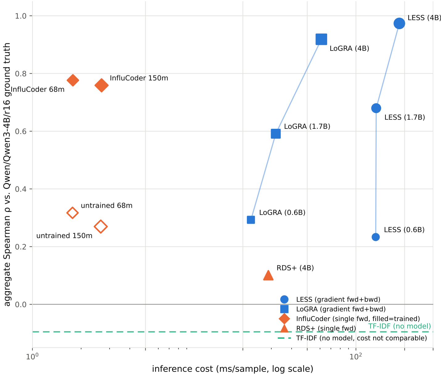
EXP1 Part 1 (BIG_GPU_FINAL) — 400x400 eval LESS r=32, LoGRA r=32 (uniform, batched)
