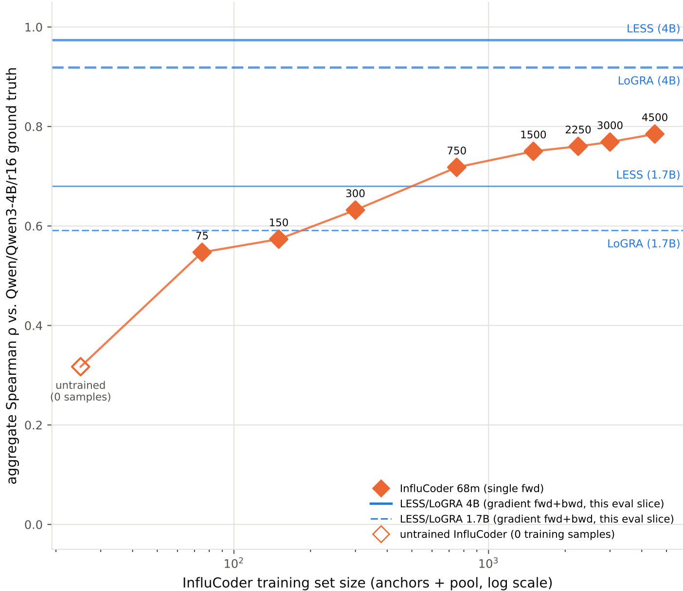
EXP1 Part 2 (BIG_GPU_FINAL) — InfluCoder scaling, 400x400 eval epochs=8, hard_ratio=0.0, lr=5e-05
