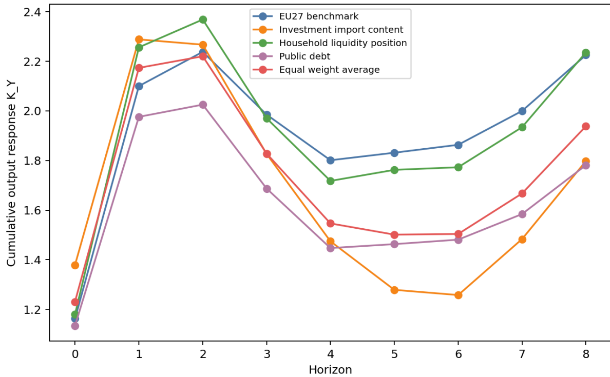
Figure 2: Cumulative output response paths K_Y(h) from impact through the eighth year. The figure plots the EU27 benchmark, the investment import content Polish evaluation, the household liquidity position Polish evaluation, the public debt Polish evaluation, and the equal weight Polish average.
