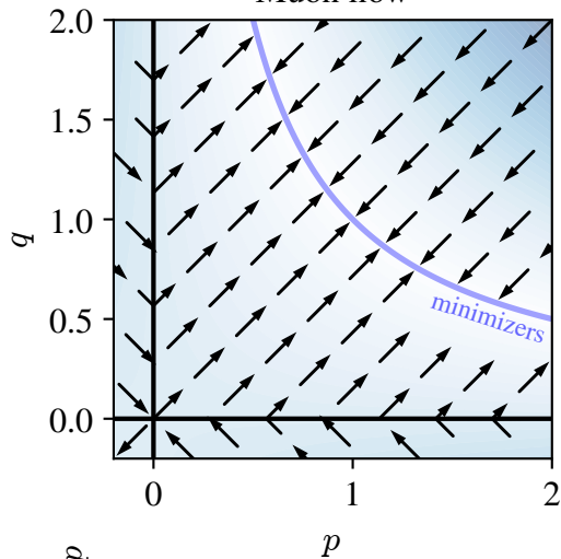
Muon flow
