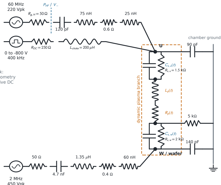
(a) Chamber section and measurement planes (b) Solved ngspice electrical schematic
