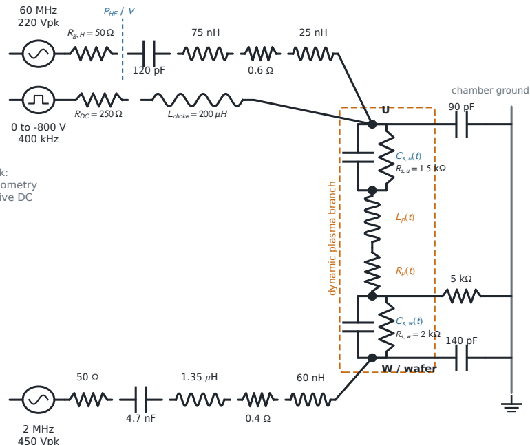
(a) Chamber section and measurement planes (b) Solved ngspice electrical schematic
